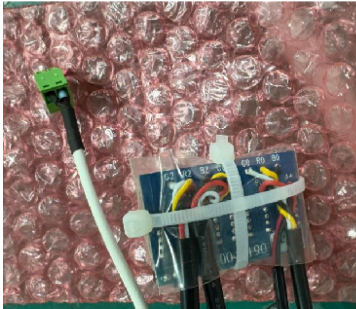
5. USE A BUBBLE BAG(ITEM410) TO HOLD THE BOARD AND COAX CABLE
