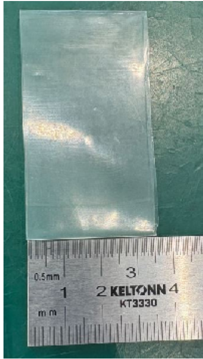
1. CUT A PIECE OF HEAT SHRINK TUBE LENGTH OF 35mm(ITEM400)
