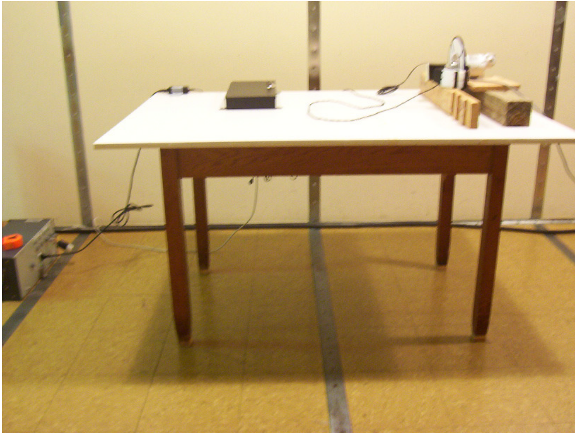
Source Tagging Tester – Conducted Emission Test Setup
