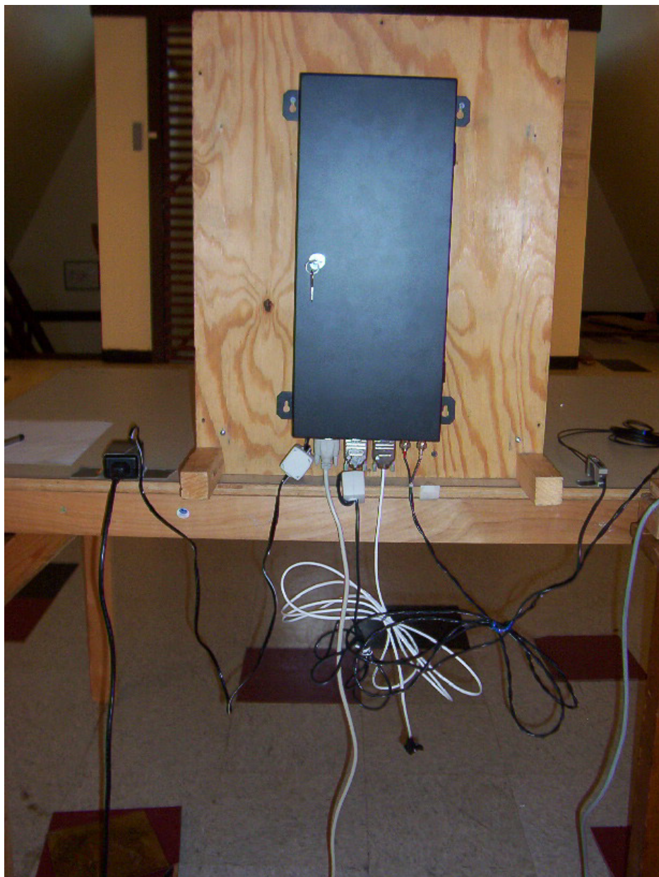
Source Tagging Tester – Radiated Emission Test Setup – Front View Vertically Mounted
