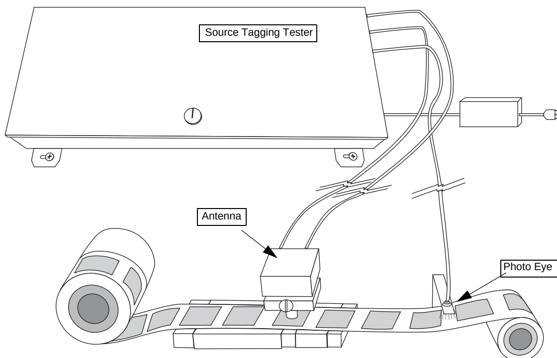
Figure 1.1 Sample Layout
