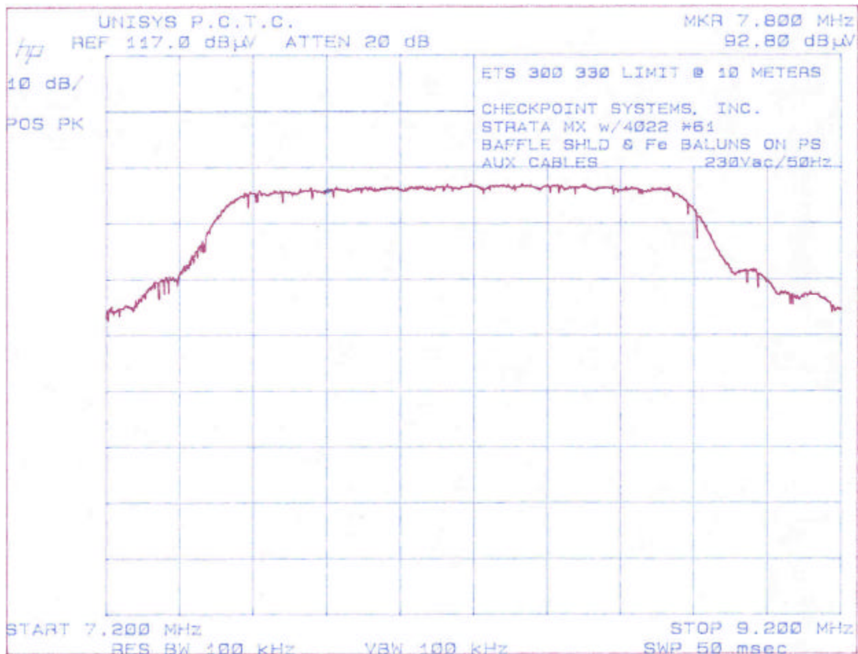
Photo 6 – Bandwidth Plot
