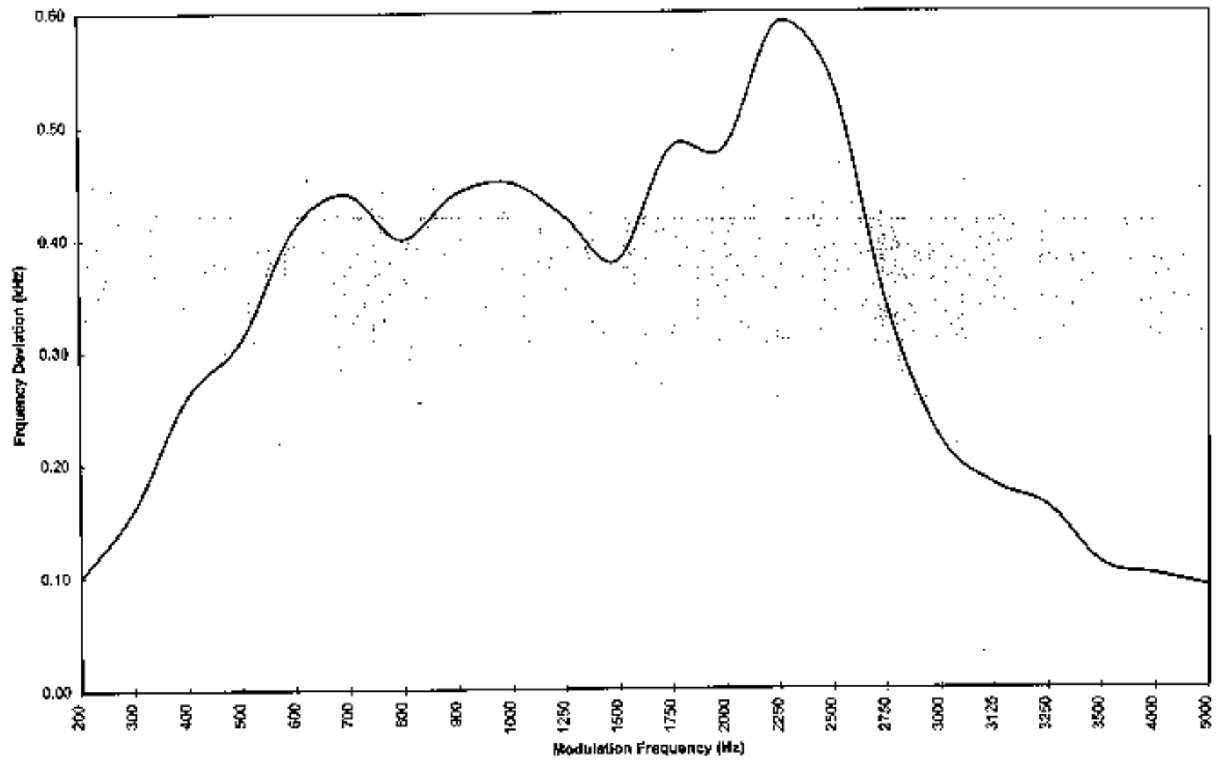
Modulation Frequency Response
