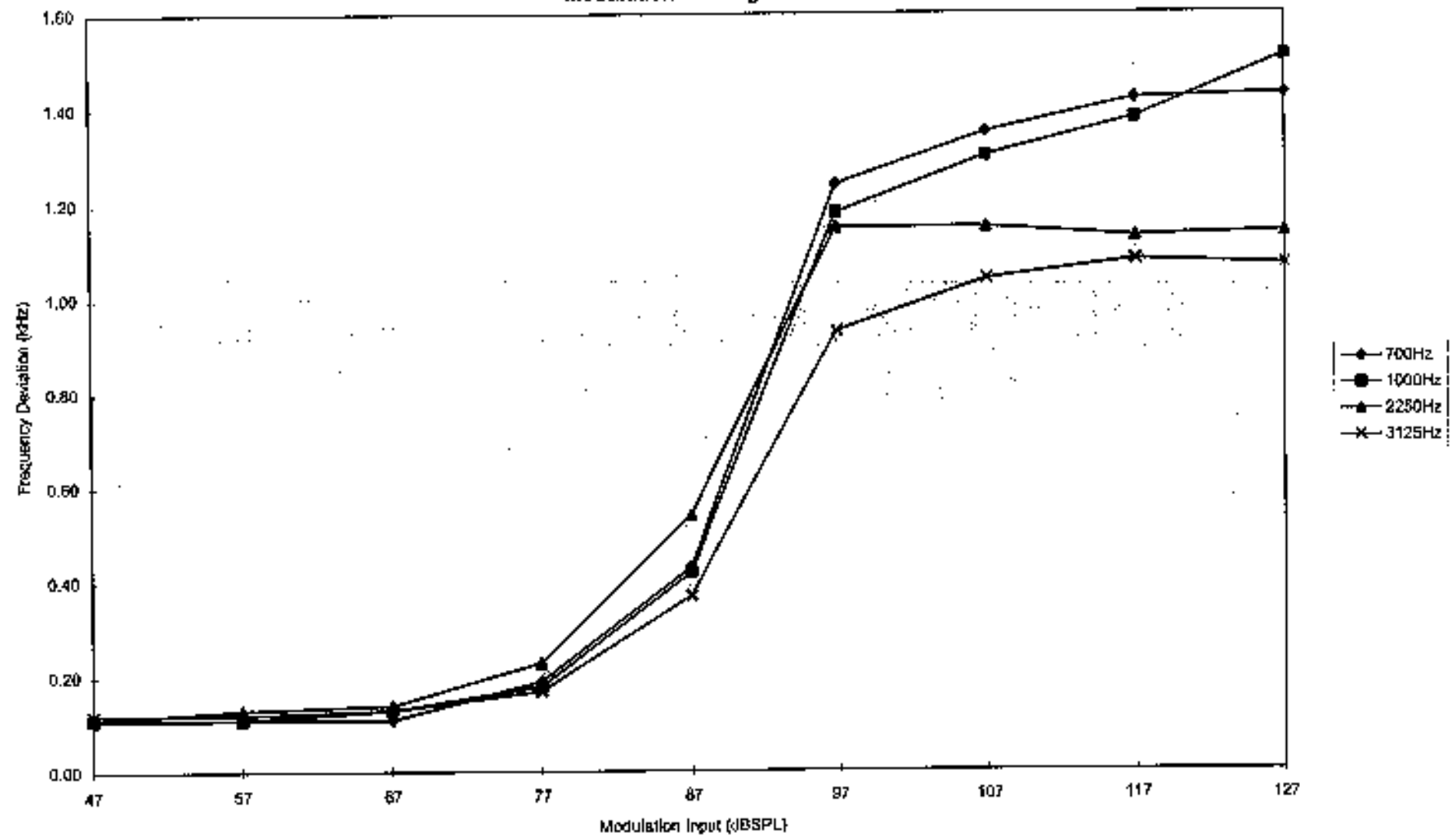
Modulation Limiting Characteristic
