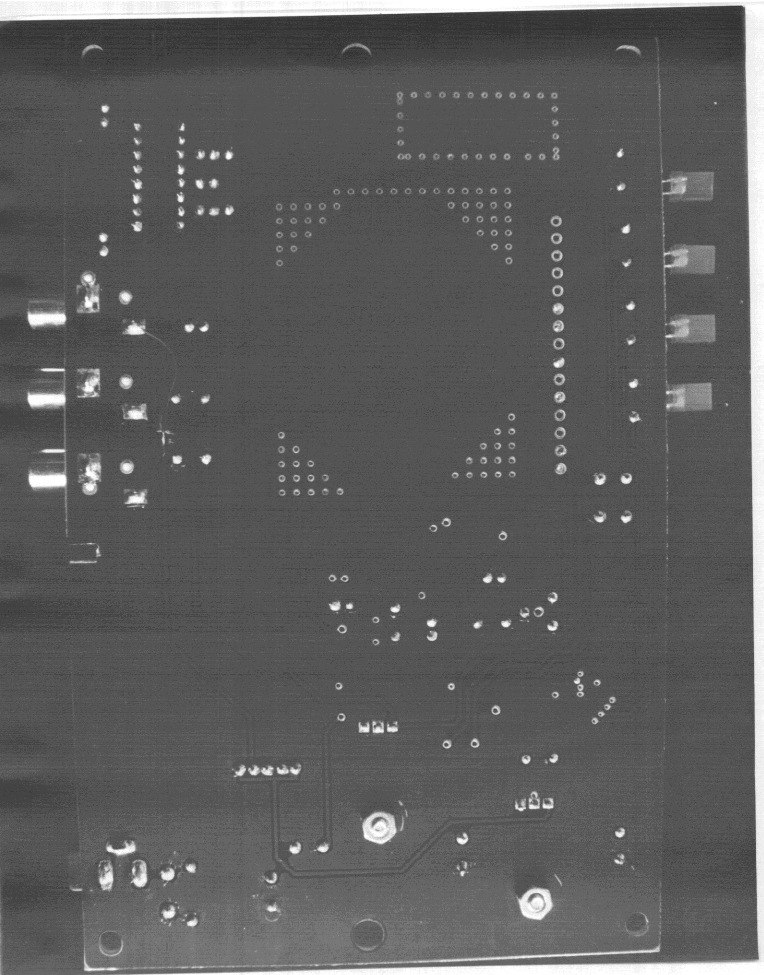
Solder View of Main Board
