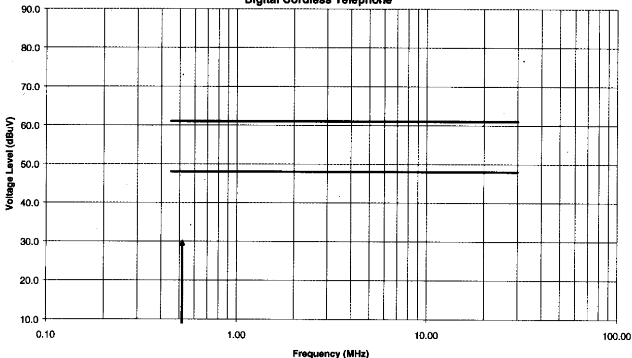
AC Conducted Emissions - Line #1 (Hot) Ultratech Engineering Labs Inc. Daewoo Telecom Ltd. Digital Cordless Telephone
