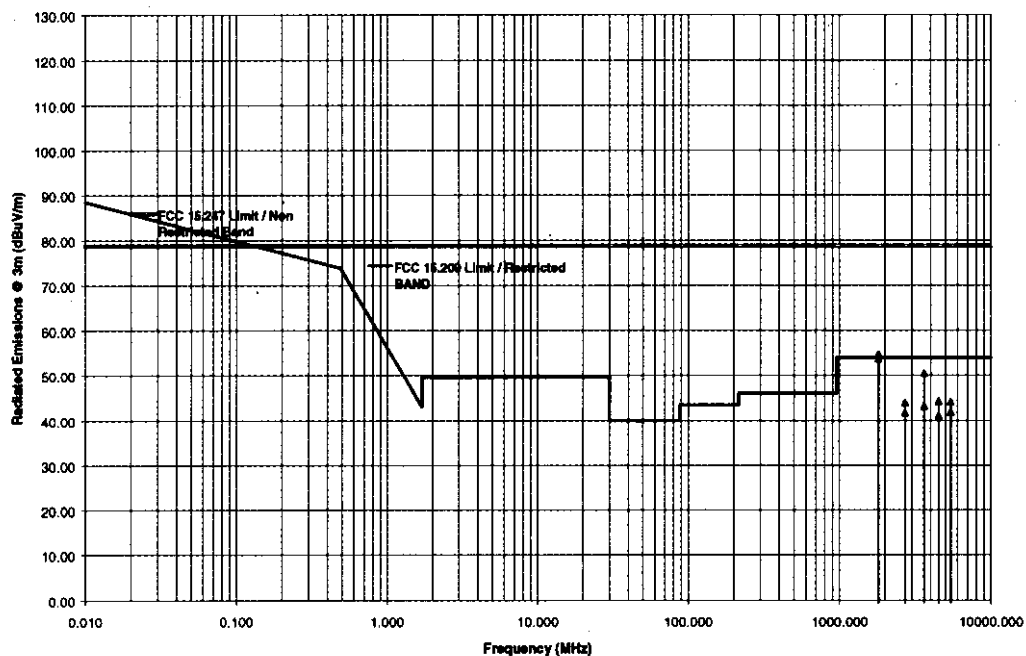
Transmitter Radiated Emissions Measurements at 3 Meter OETS Daewoo Telecom Ltd. Digital Cordless Telephone (Base) TRANSMIT Freq.: 904.2MHz
