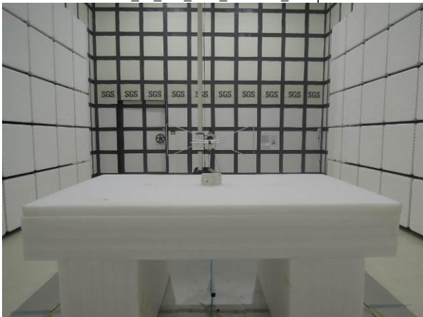
FCC_15_225_NFC_Radiated_Setup
