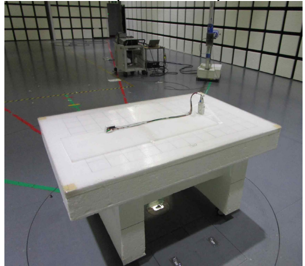
Rear (Above 1 GHz)
