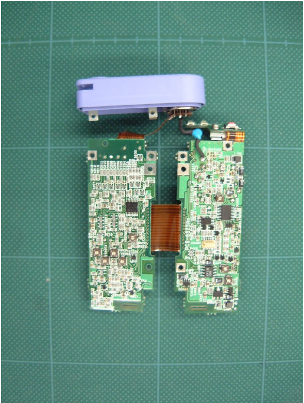
PCB Solder Side
