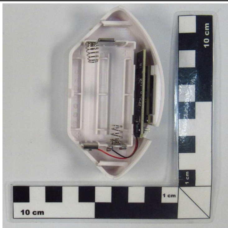
EUT opened
