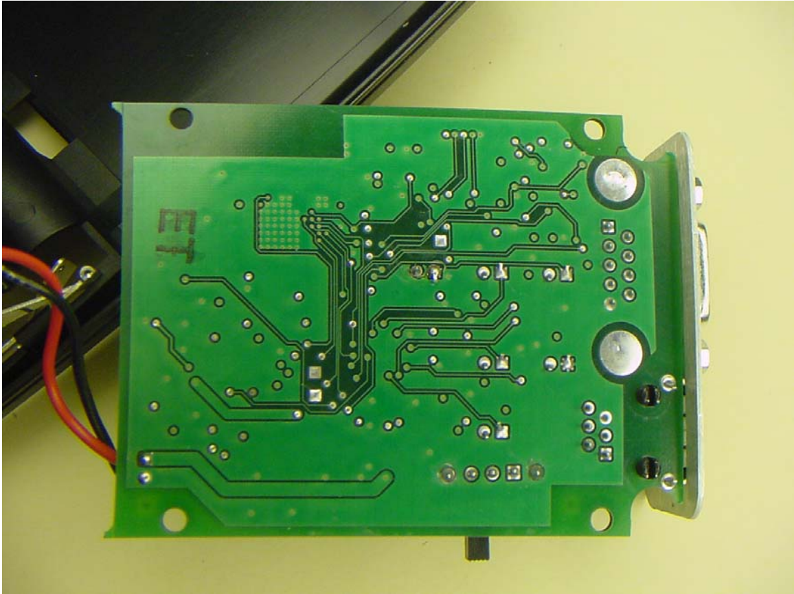
263-05 TAC ROAMIO PCB Solder Side
