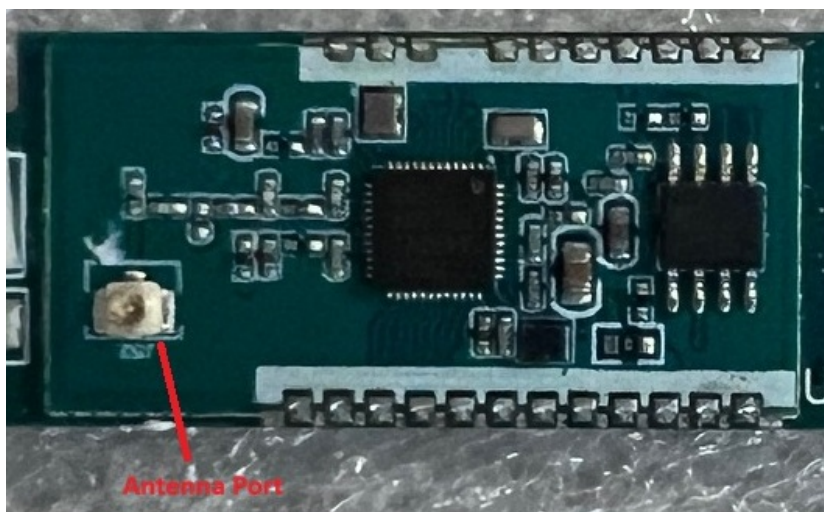
EUT- Component Top Side View
