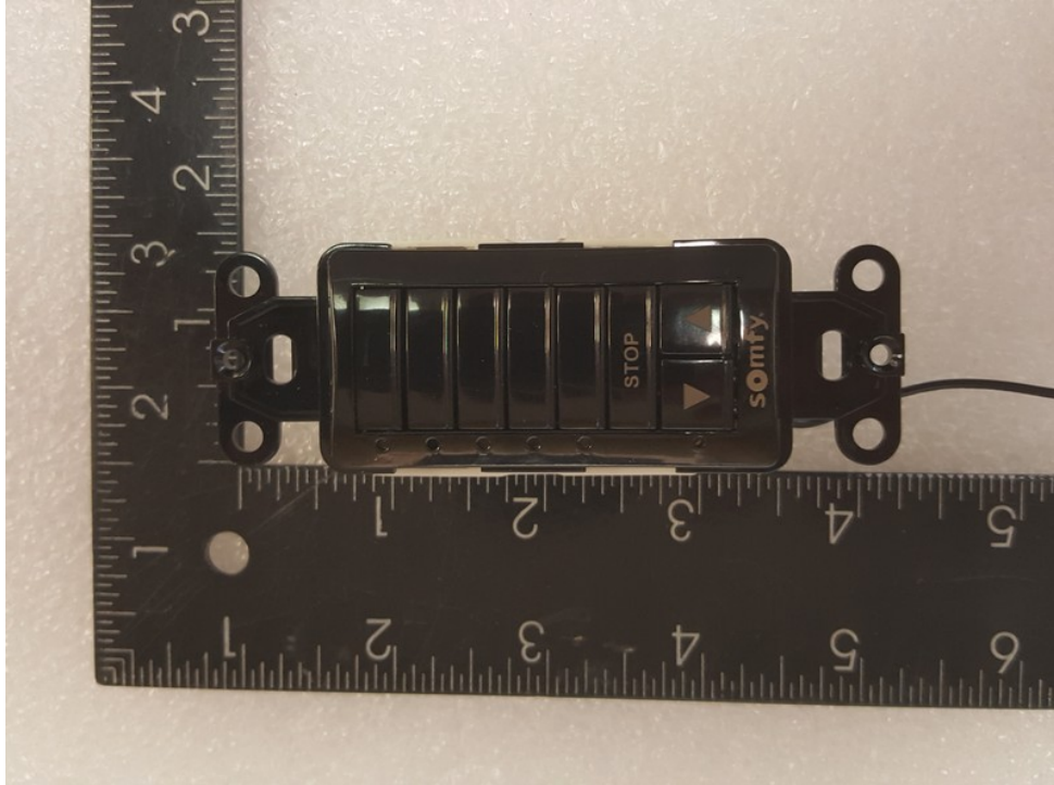
Figure 7.1 Top/Front View (Dimension)
