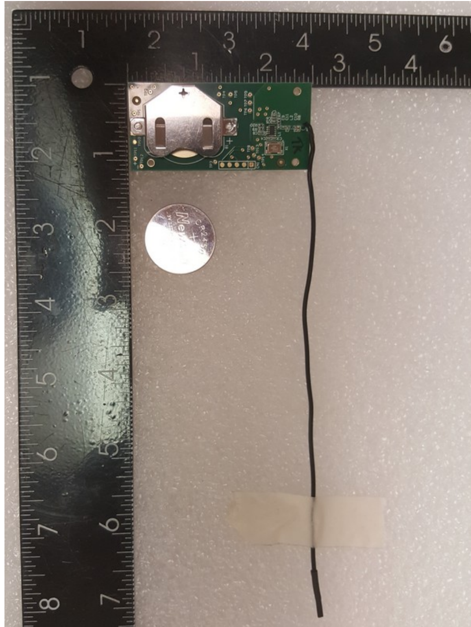
Figure 7.9 EUT Antenna Size
