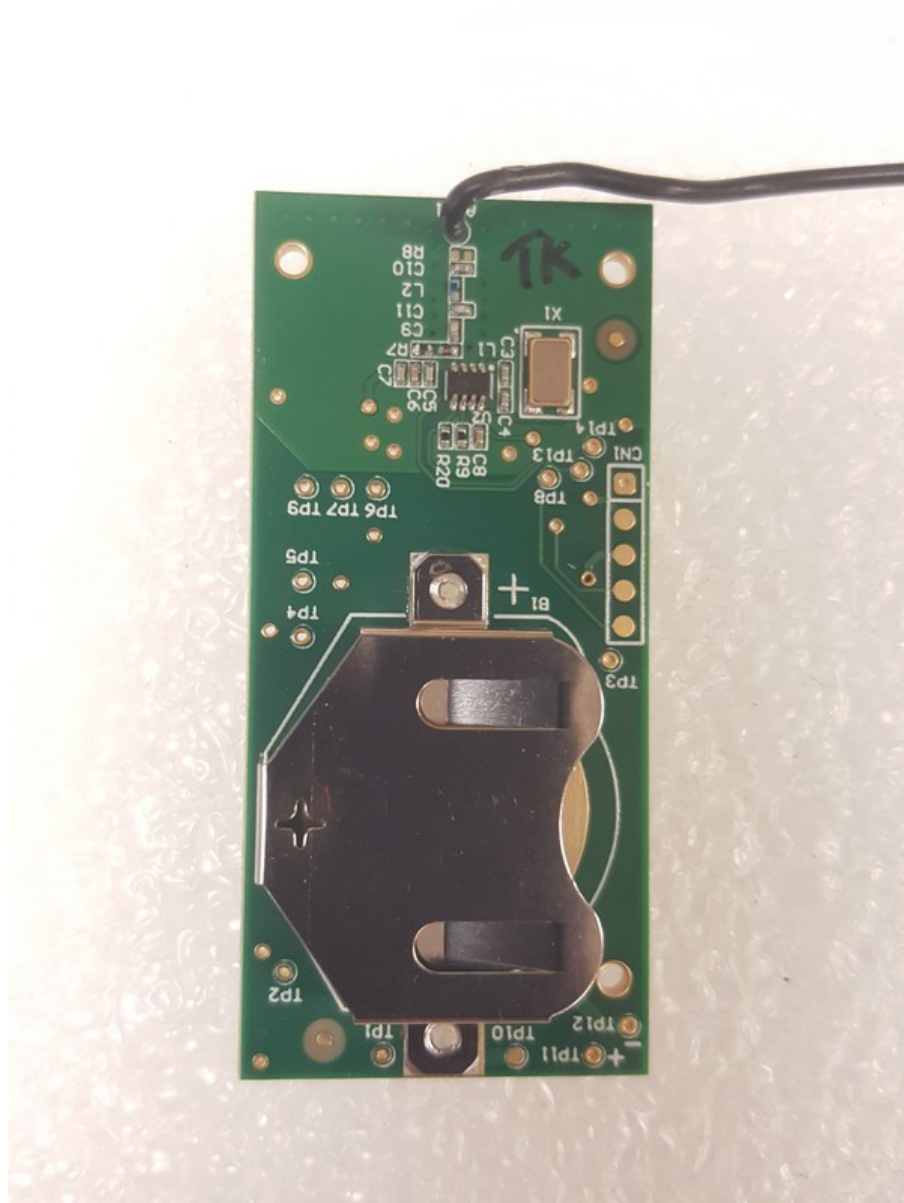
Figure 7.7 EUT components side
