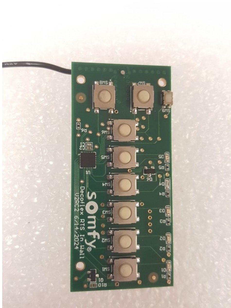
Figure 7.8 EUT Push Button side
