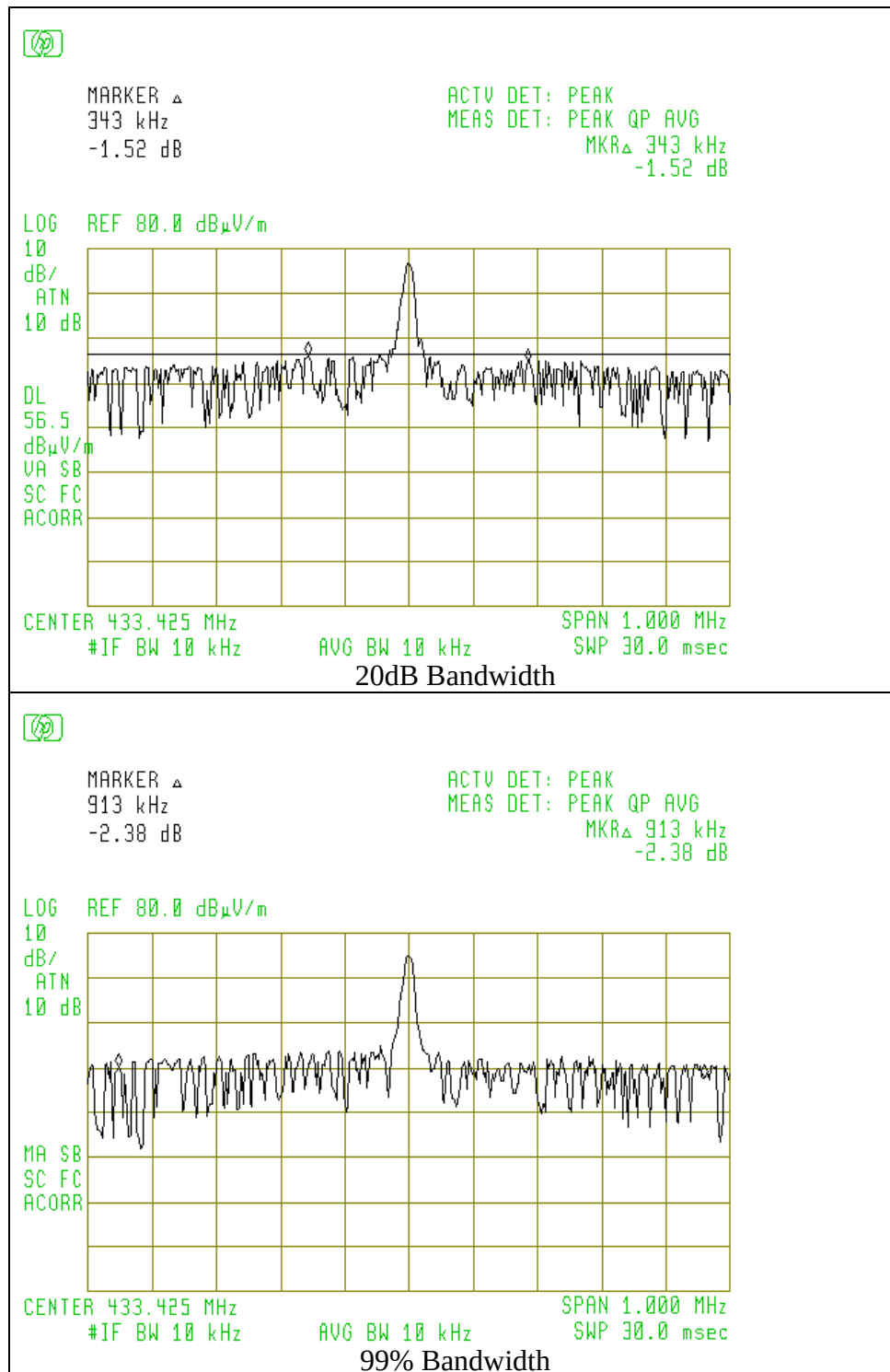
Figure 6.1 Occupied Bandwidth
