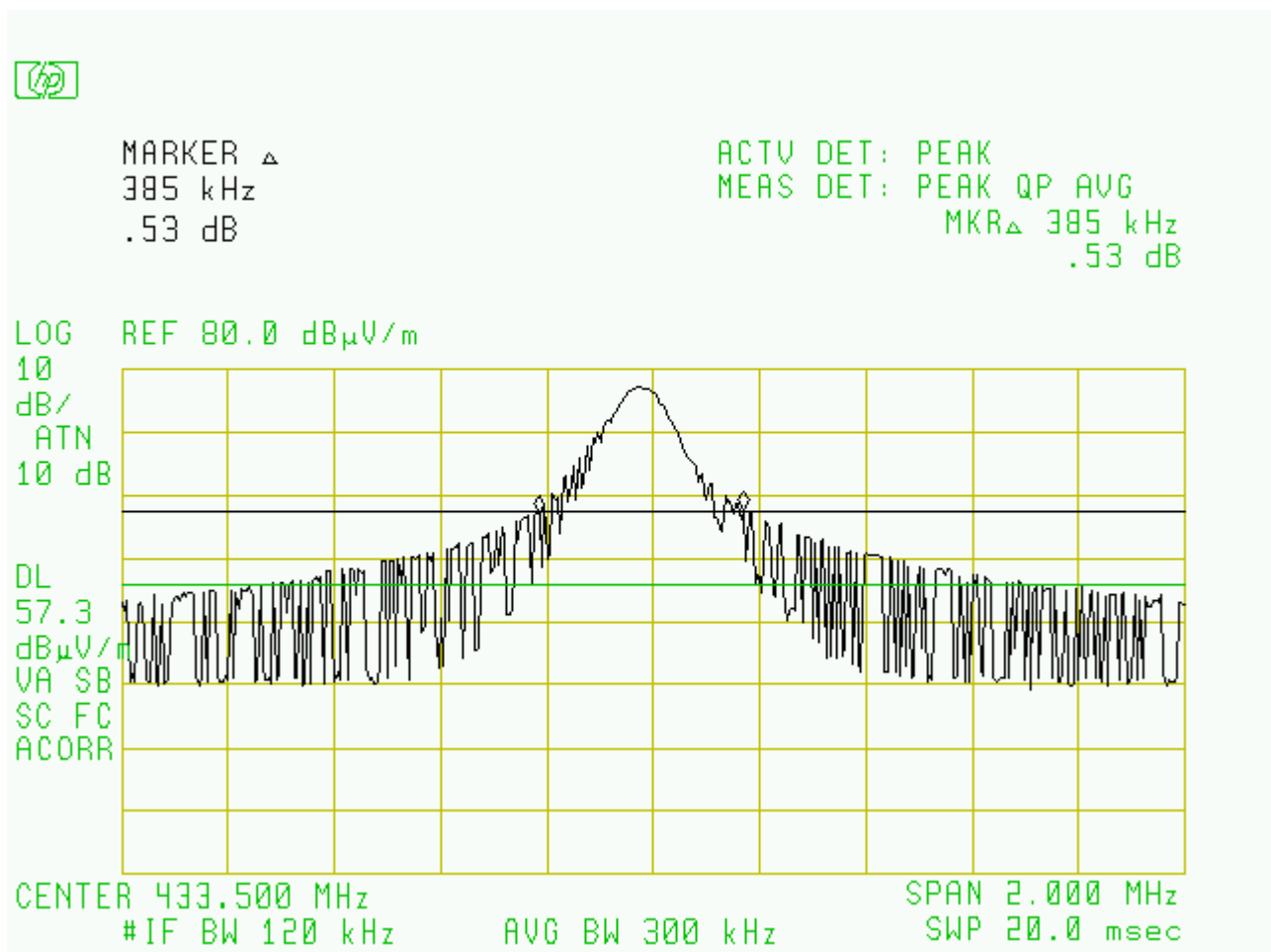
Figure 6.1 Occupied Bandwidth
