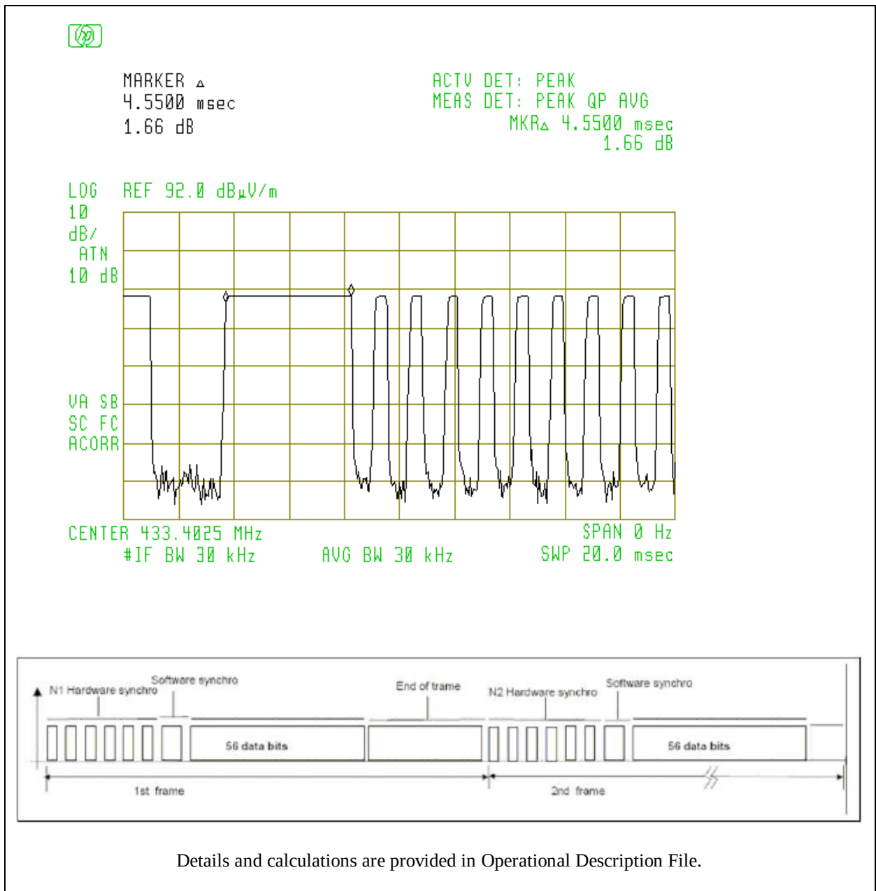
Figure 6.2 Pulse Train Timing
