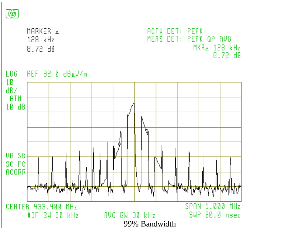
Figure 6.1 Occupied Bandwidth
