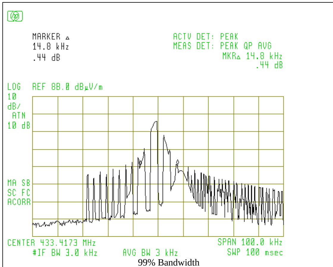
Figure 6.1 Occupied Bandwidth
