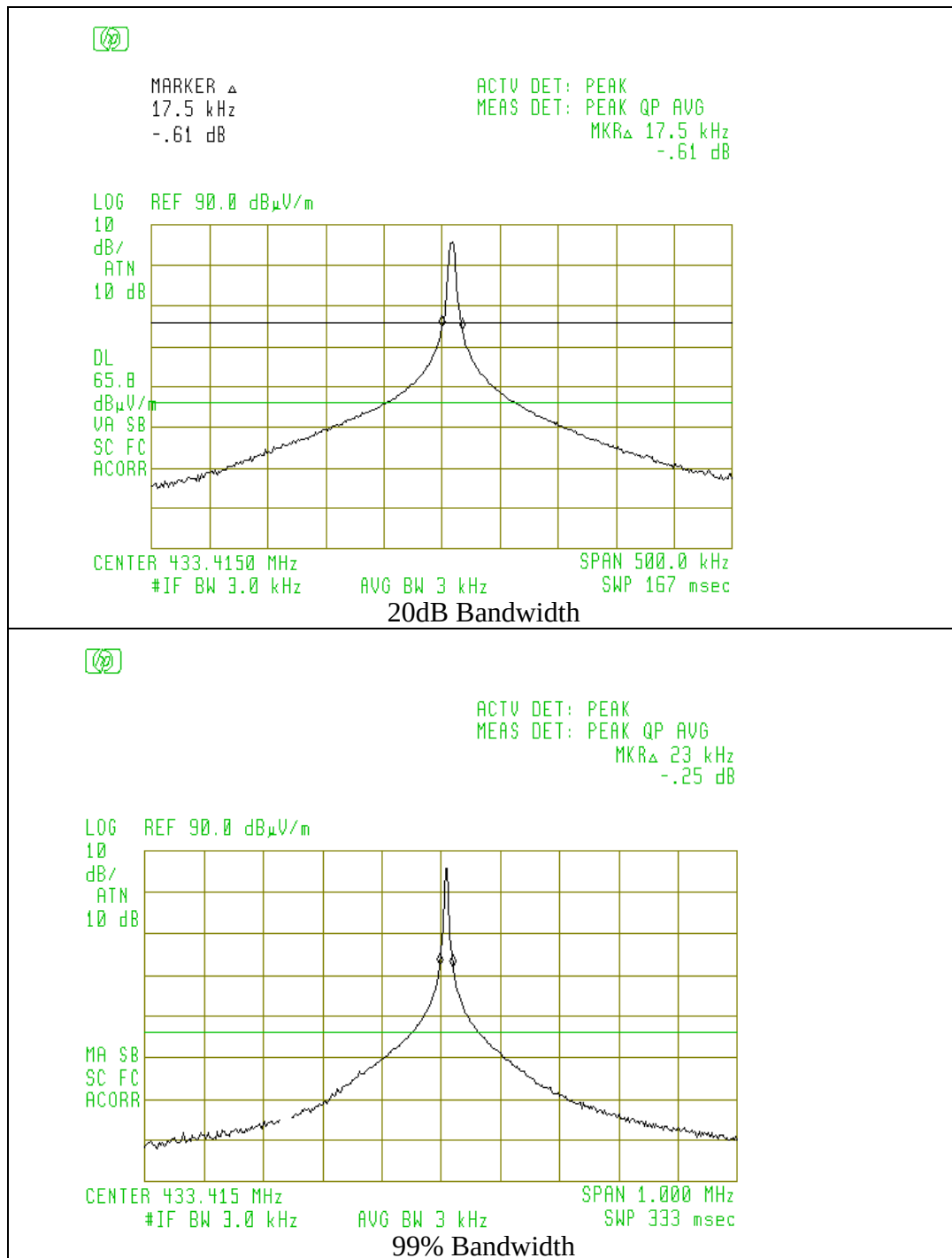
Figure 6.1 Occupied Bandwidth
