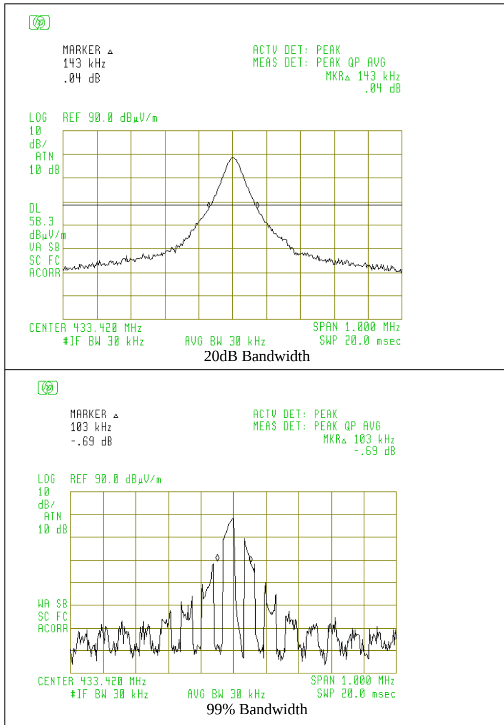
Figure 6.1 Occupied Bandwidth
