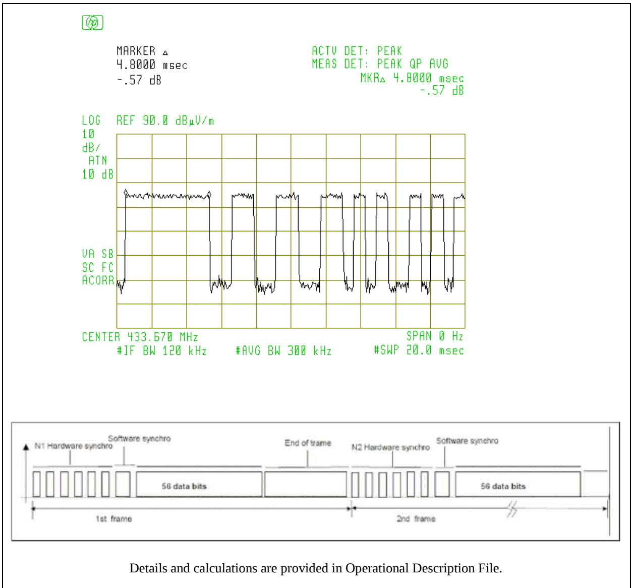
Figure 6.2 Pulse Train Timing
