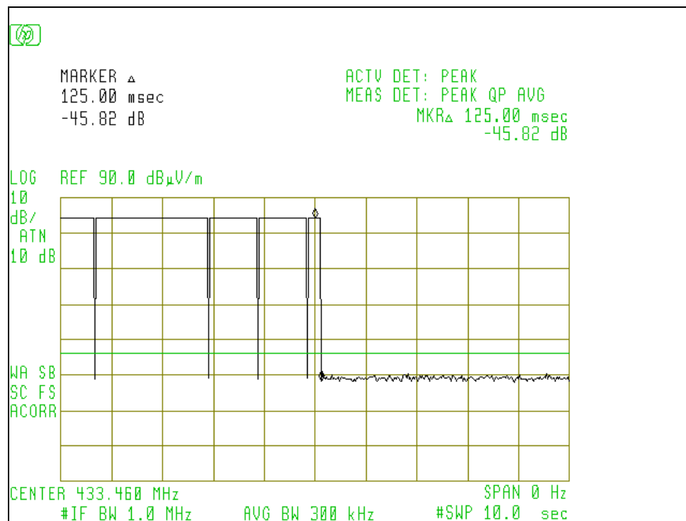
Tx stopped within 5s after button released
