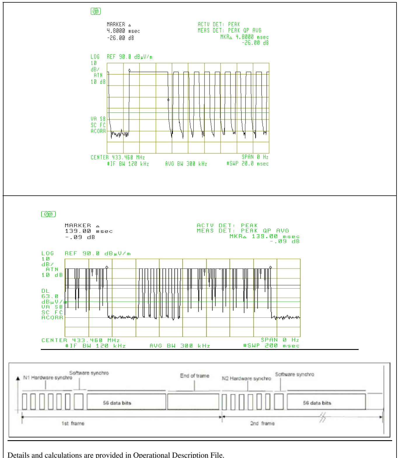
Figure 6.2 Pulse Train Timing
