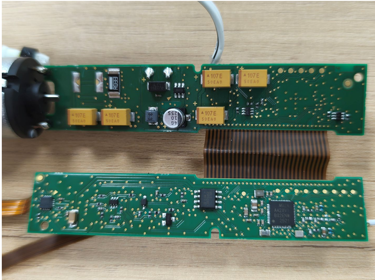
PCBA VIEW
