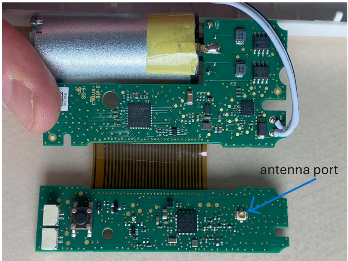
EUT PCB Back View
