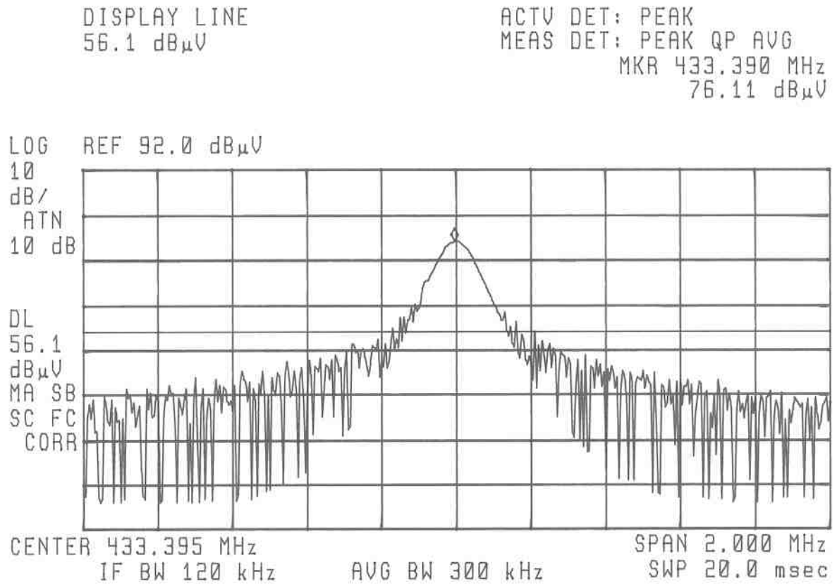
Figure 5.2 Occupied Bandwidth
