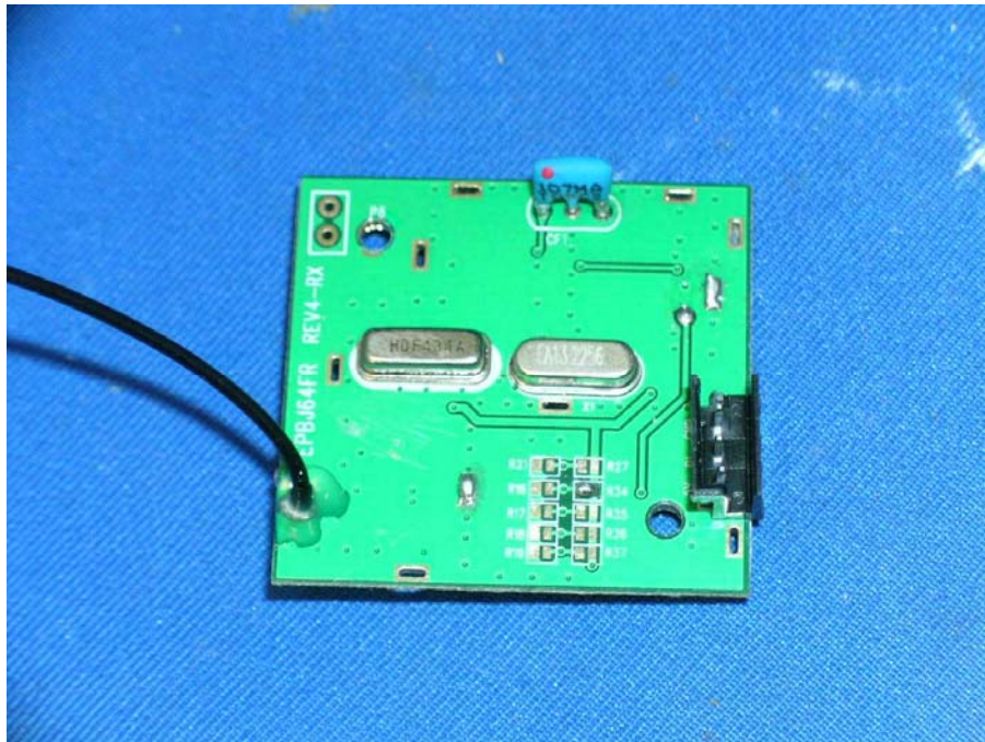
433MHz Receiver solder side
