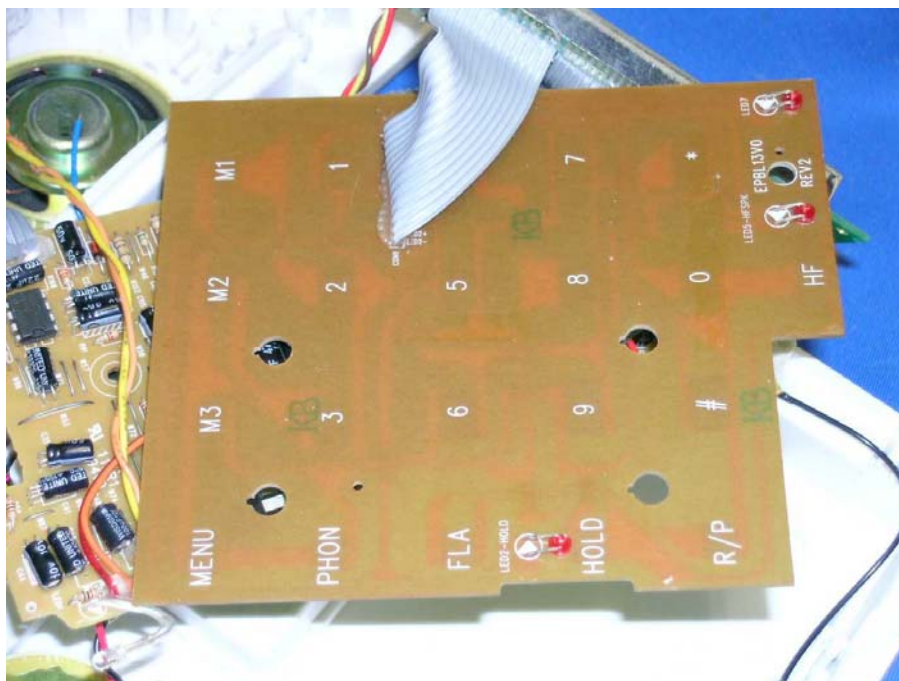
Corded Phone Keypad rear side (View 2)
