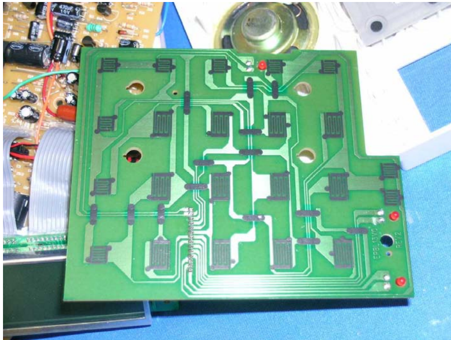
Corded Phone Keypad front side
