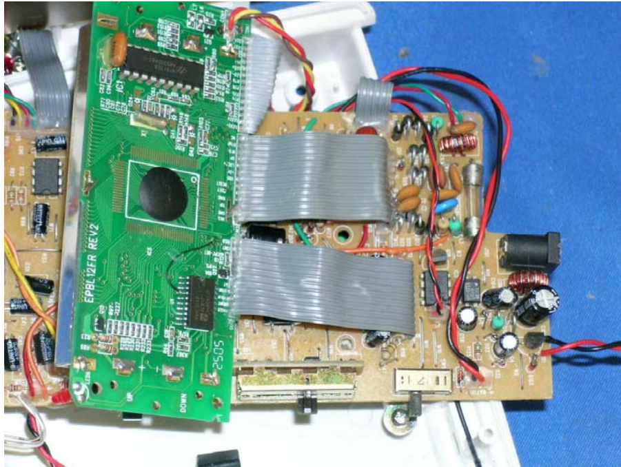
Corded Phone Main PCB component side (View 2)
