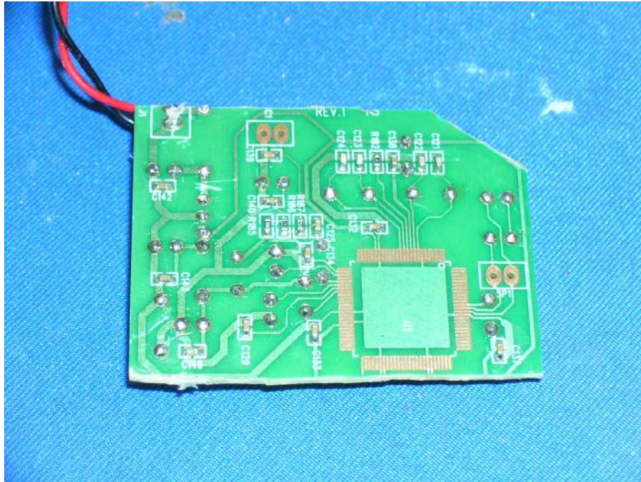
Corded Phone Oscillator solder side
