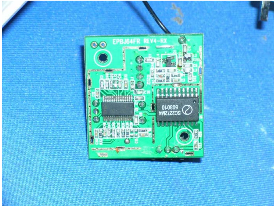
433MHz Receiver component side
