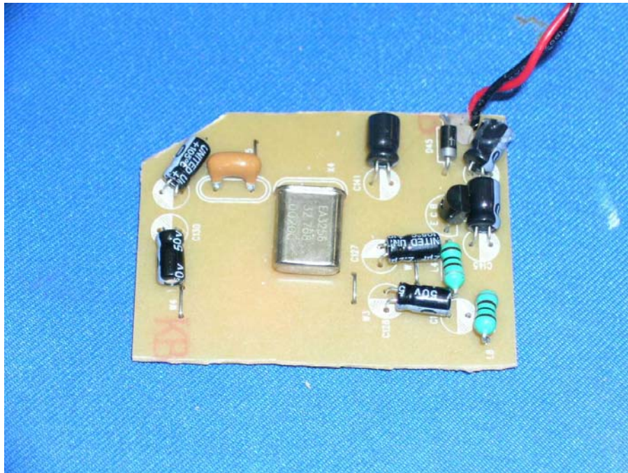
Corded Phone Oscillator component side
