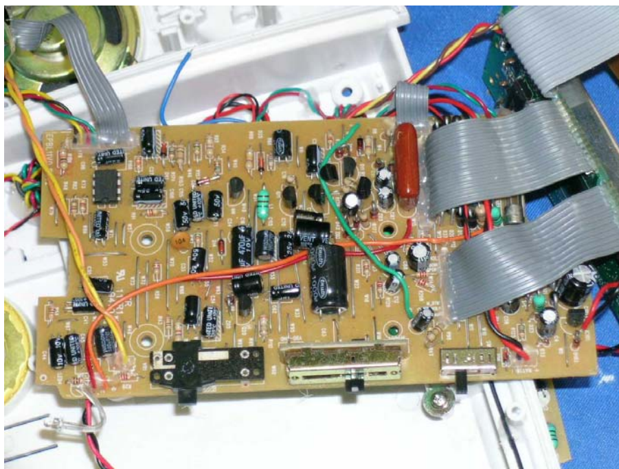
Corded Phone Main PCB component side (View 1)
