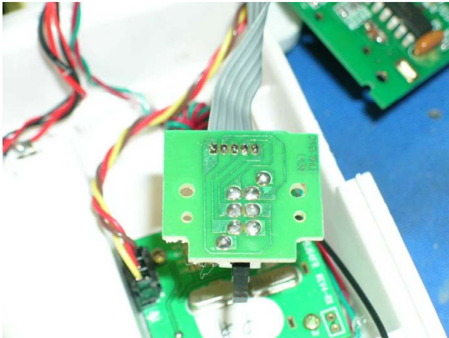
Corded Phone Hook Switch solder side
