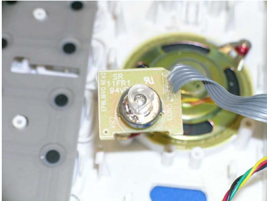
Corded Phone's Headset Volume Control component side
