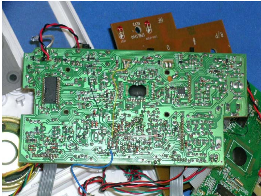
Corded Phone Main PCB solder side
