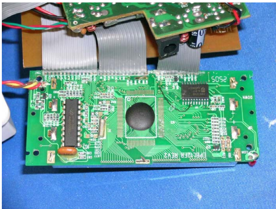
Corded Phone LCD Display front side (View 2)
