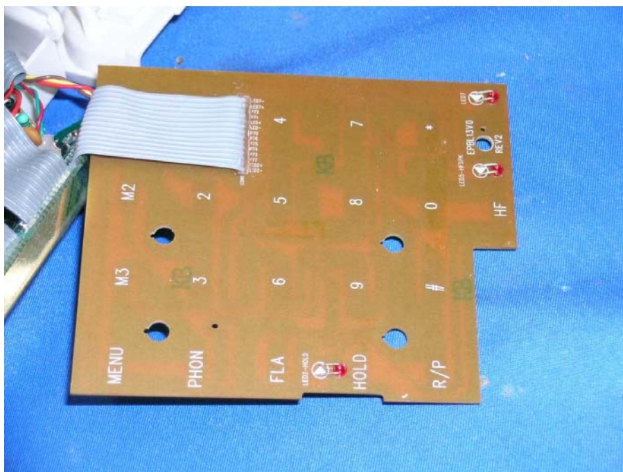
Corded Phone Keypad rear side (View 1)
