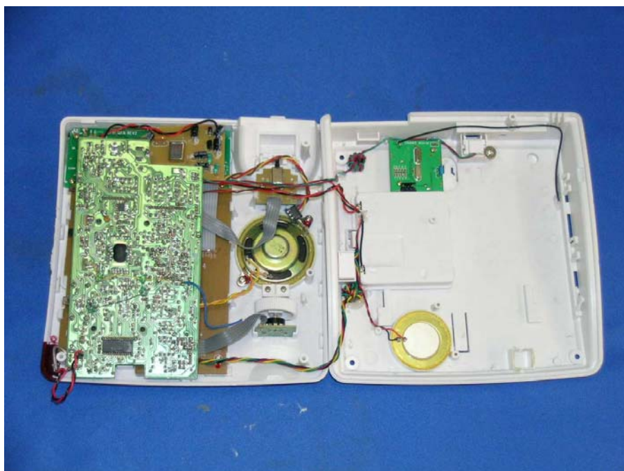
Corded Phone with 433MHz receiver assembly
