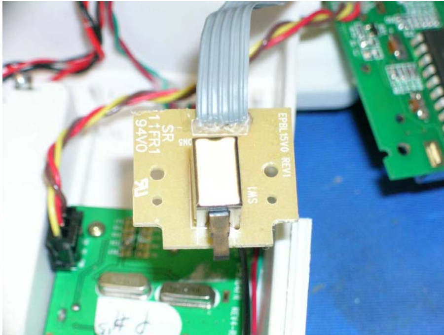
Corded Phone Hook Switch component side
