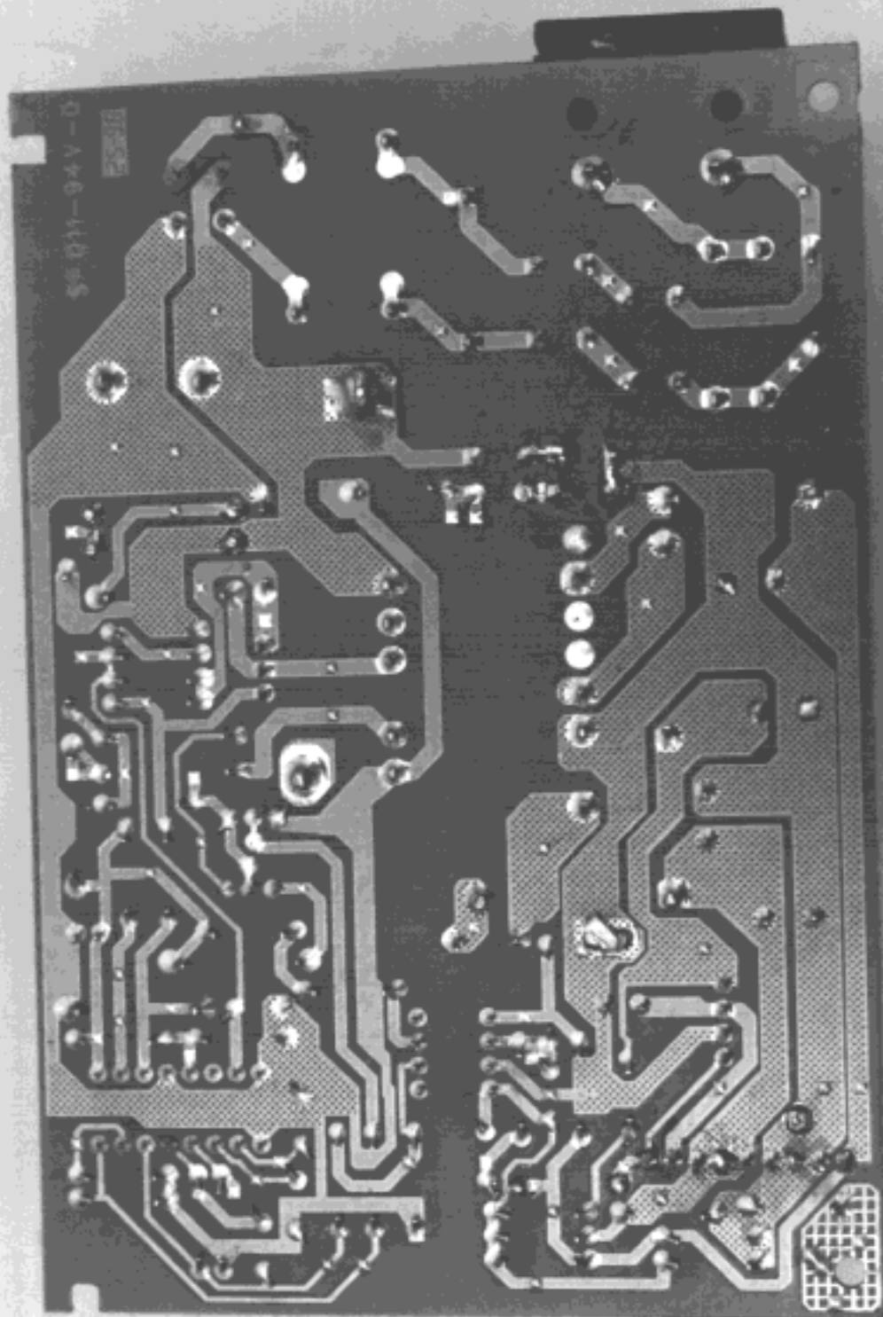
Fig. 8.6 Power Supply Unit P.W.A. - Foil side
