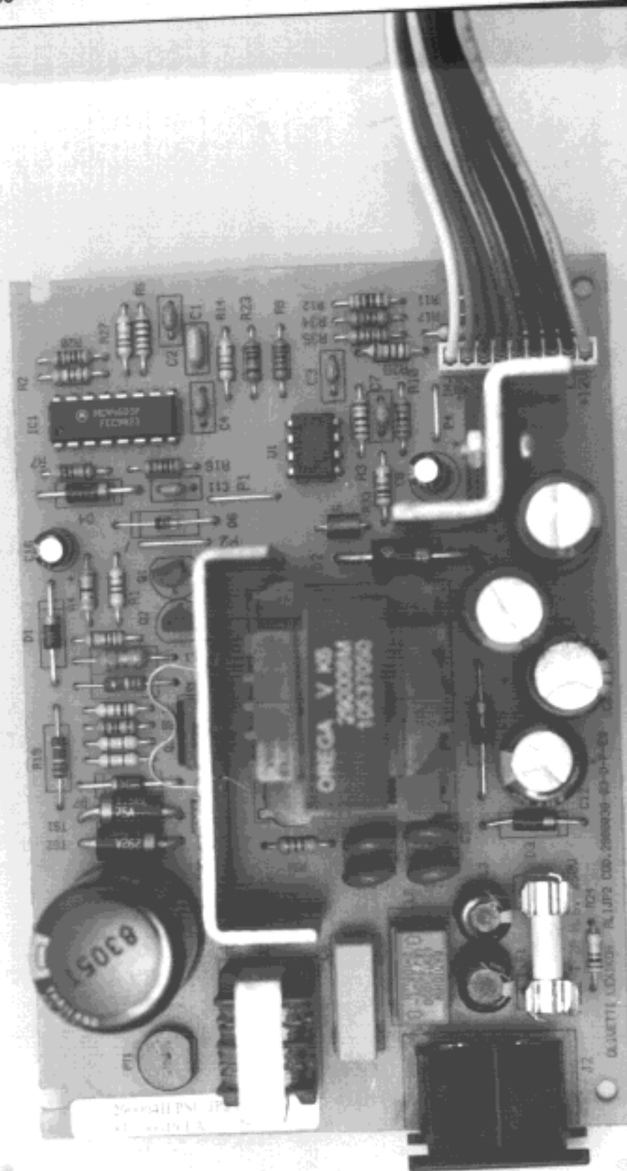
Fig. 8.5 Power Supply Unit P.W.A. - Components side
