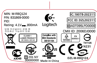
Label for Corbusier Rev03 PDM-645844-0000
