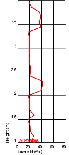
Height Plot ( 128.572745826 MHz )
