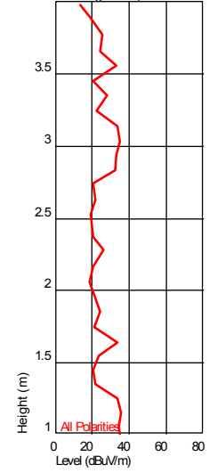
Height Plot ( 74.012625357 MHz )
