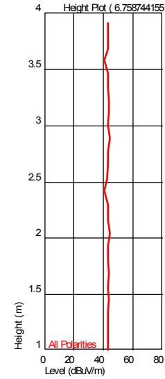
Height Plot ( 6.758744155 GHz )
