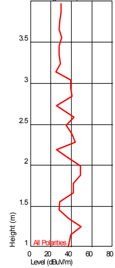
Height Plot ( 782.338075958 MHz )
