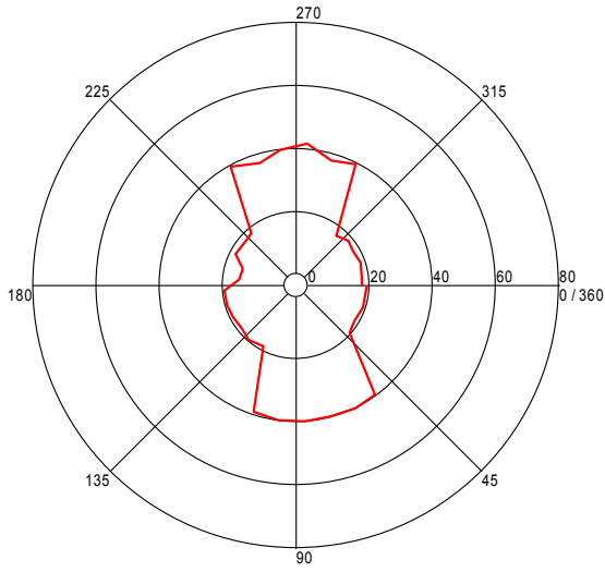
Turntable Plot ( 51.742083693 MHz )
