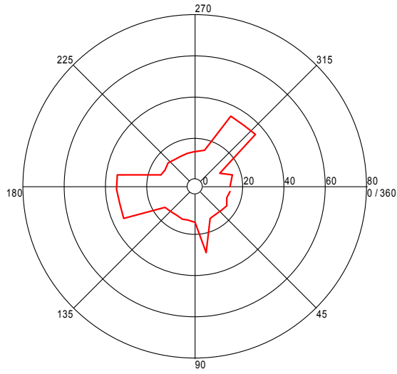
Turntable Plot ( 74.156112331 MHz )
