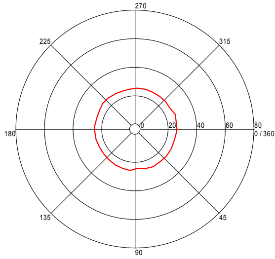
Turntable Plot ( 71.994789405 MHz )
