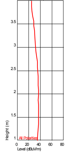
Height Plot ( 504.045691148 MHz )
