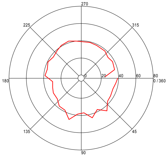
Turntable Plot ( 779.374348222 MHz )
