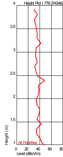
Height Plot ( 779.374348222 MHz )
