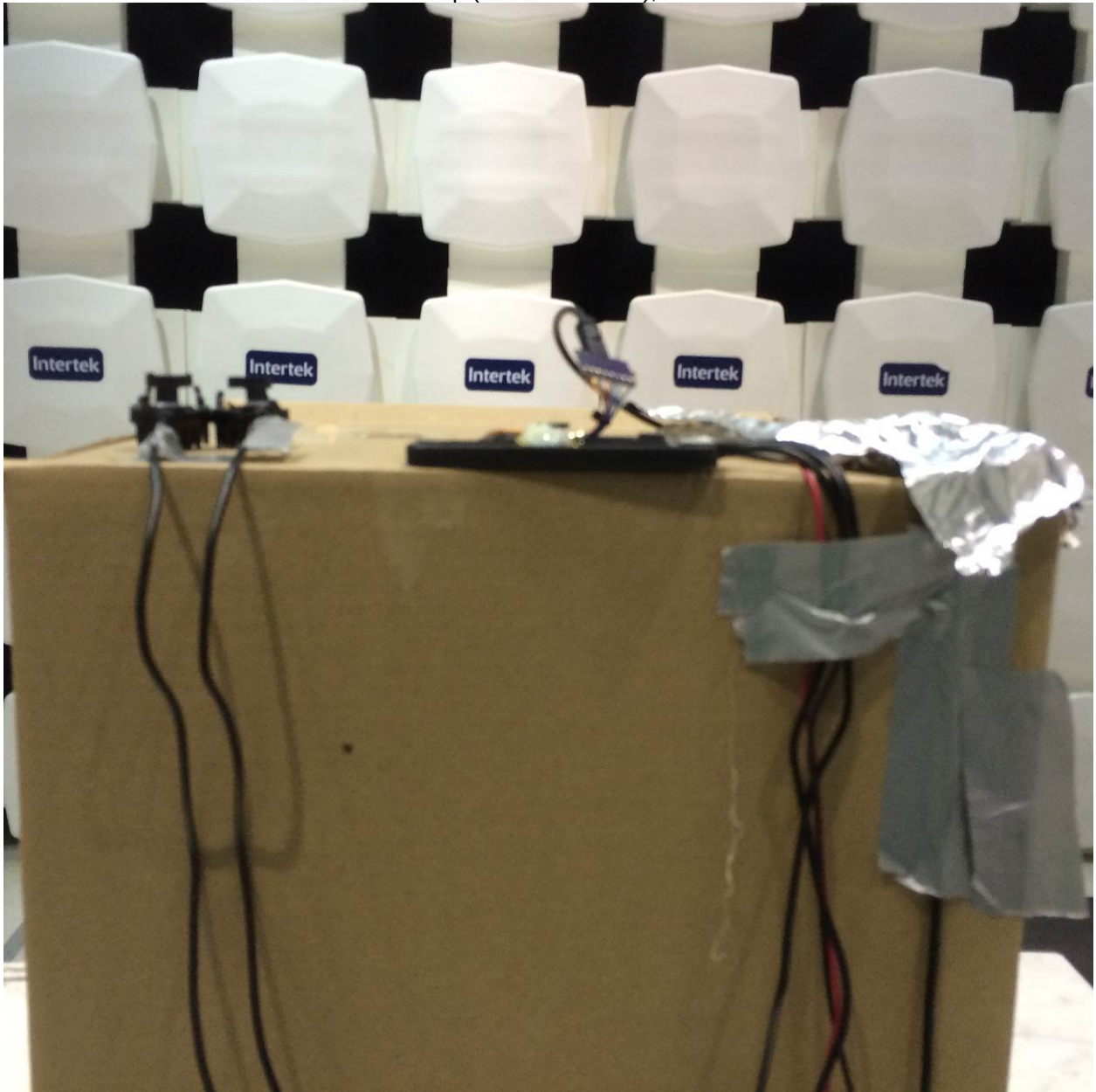
Test Setup (EUT on its back), Photo 2
