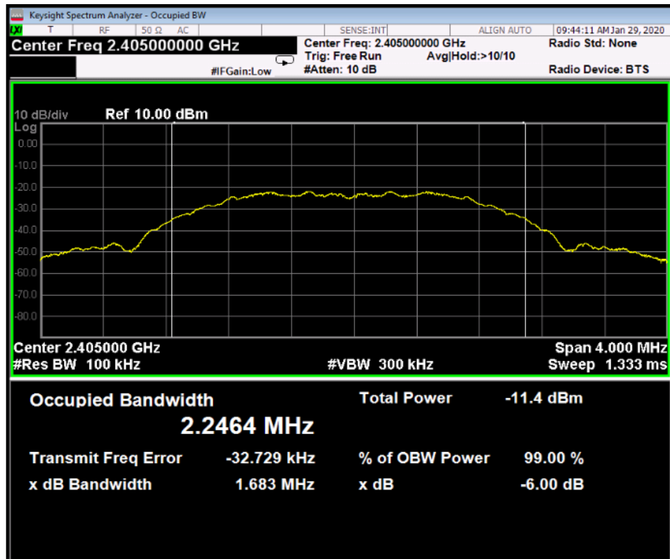
Occupied Bandwidth – Low Channel
