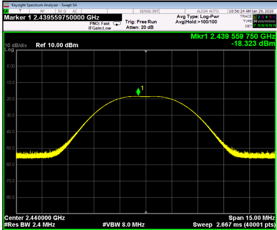
Peak Output Power – Mid Channel
