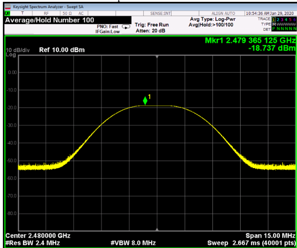
Peak Output Power – High Channel
