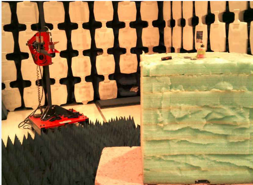
1-6GHz
