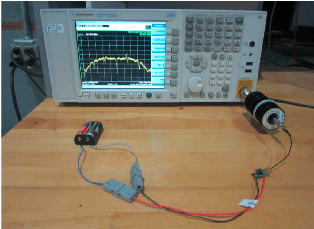
Antenna Port
