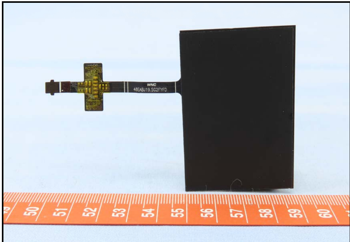
WNC antenna
