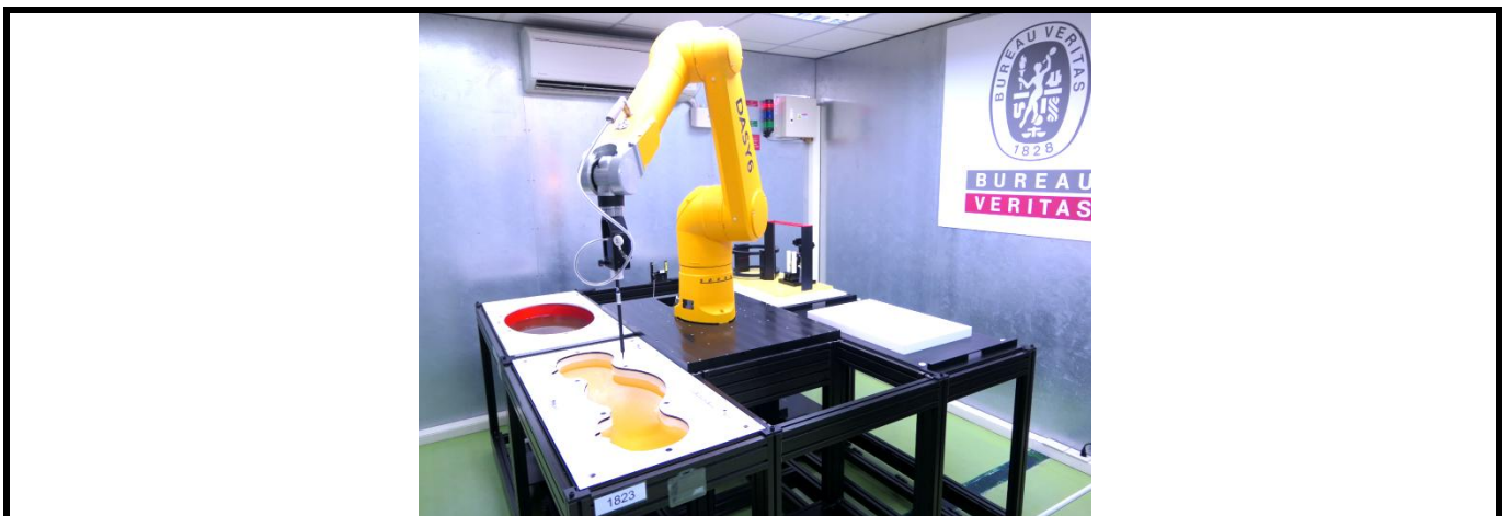
Fig-4.2 SPEAG DASY6 System
