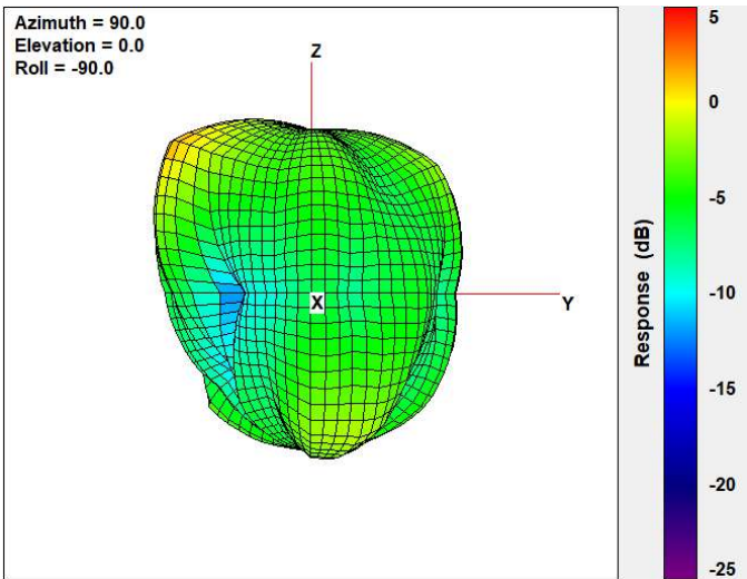
Max Antenna 3D Radiation Pattern 5150-5250 MHz
