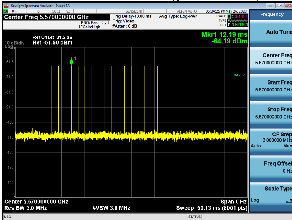
Mode 1: Transmit - 802.11ac-160MHz Radar Type 0 Calibration Plot (5570MHz)
