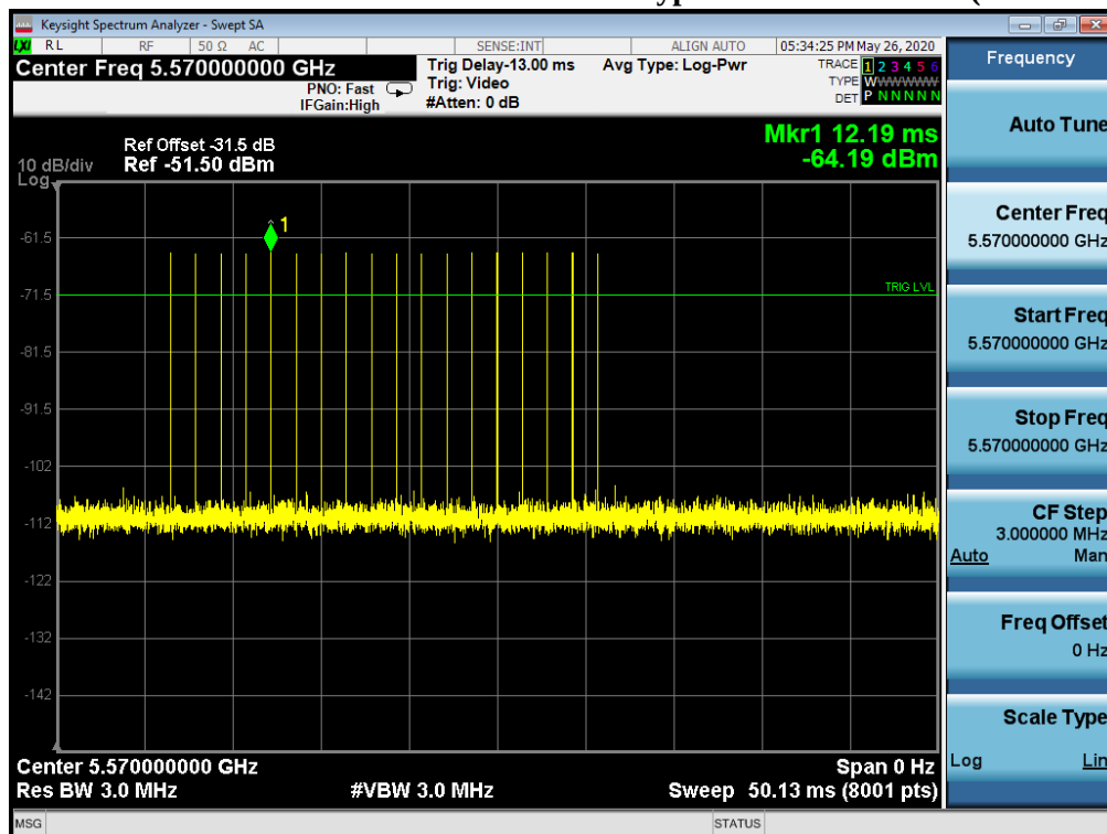
Mode 2: Transmit - 802.11ax-160MHz Radar Type 0 Calibration Plot (5570MHz)
