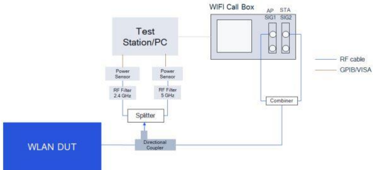
Figure 4-4 SISO (Simultaneous Transmission) – Validation test setup
