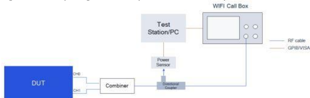
Figure 4-2 SISO (Change in Antenna) – Validation test setup
