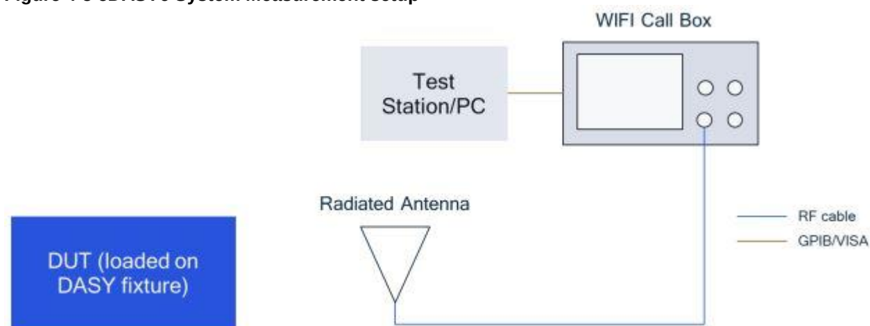
Figure 4-5 cDASY6 System Measurement setup
