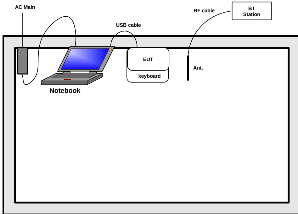
Test Setup Diagram - Radiated Below 1GHz Test (Mode 4)
