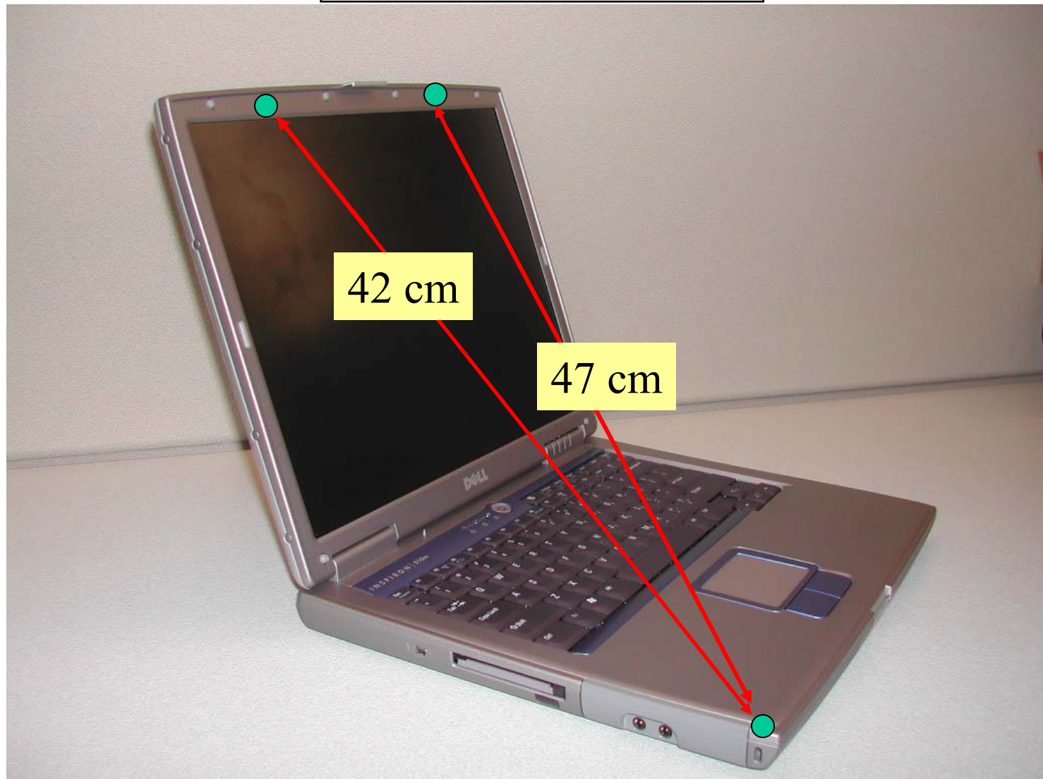
Antenna distance to BlueTooth module
