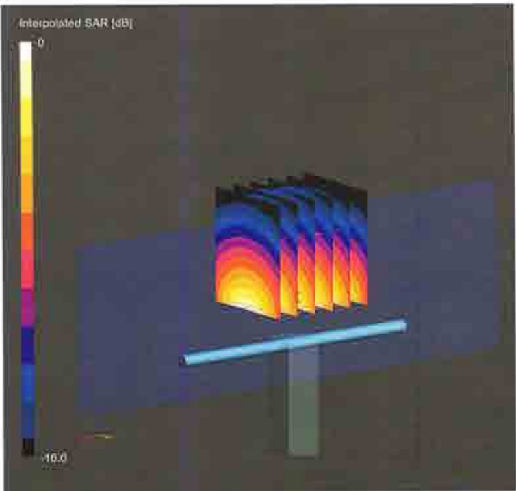
0 dB = 15.9 W/Kg
