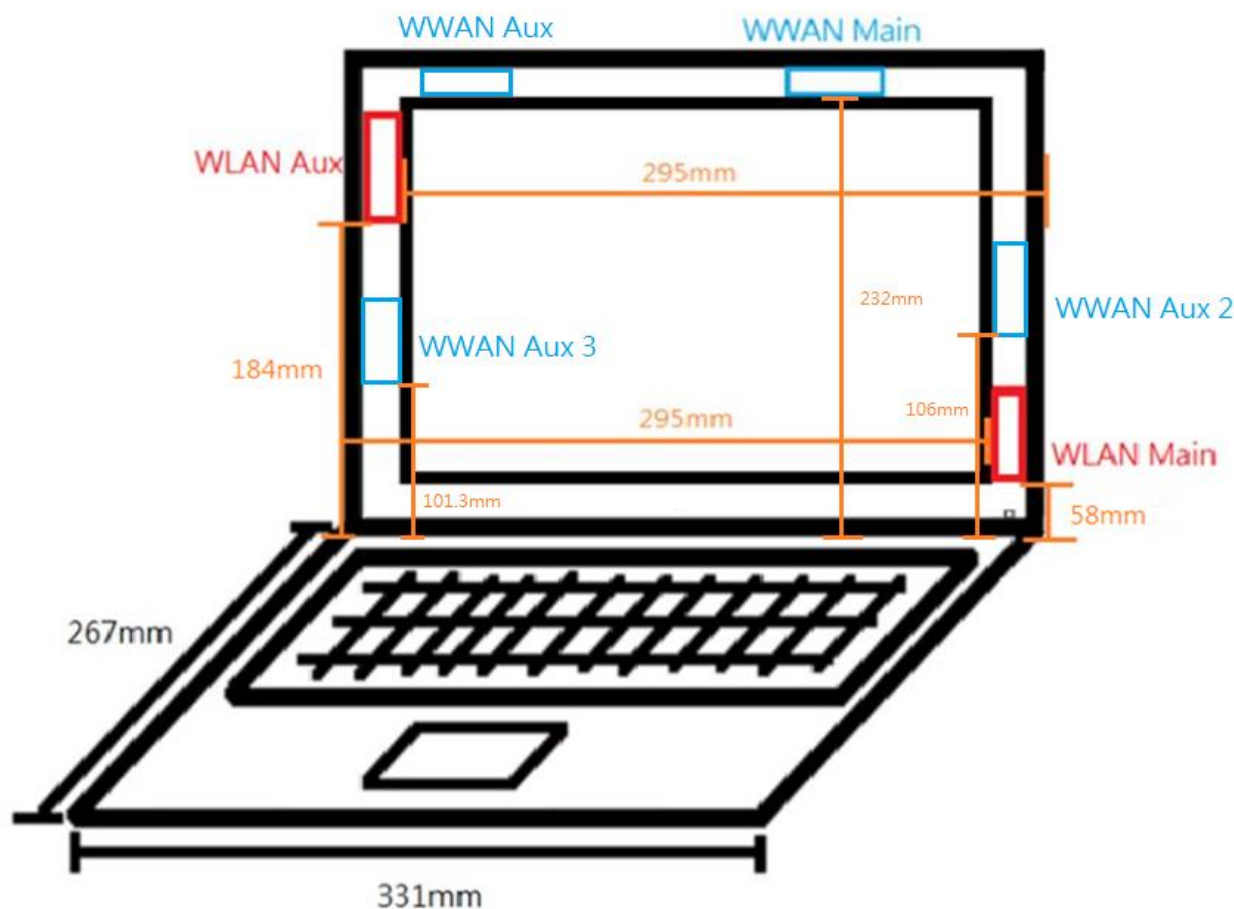
Photograph 5. Antenna position of EUT
