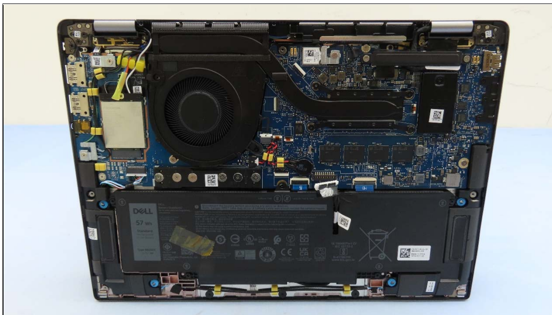
BT + WiFi module (Brand: Intel® BE200D2W, Model: BE200D2W)
