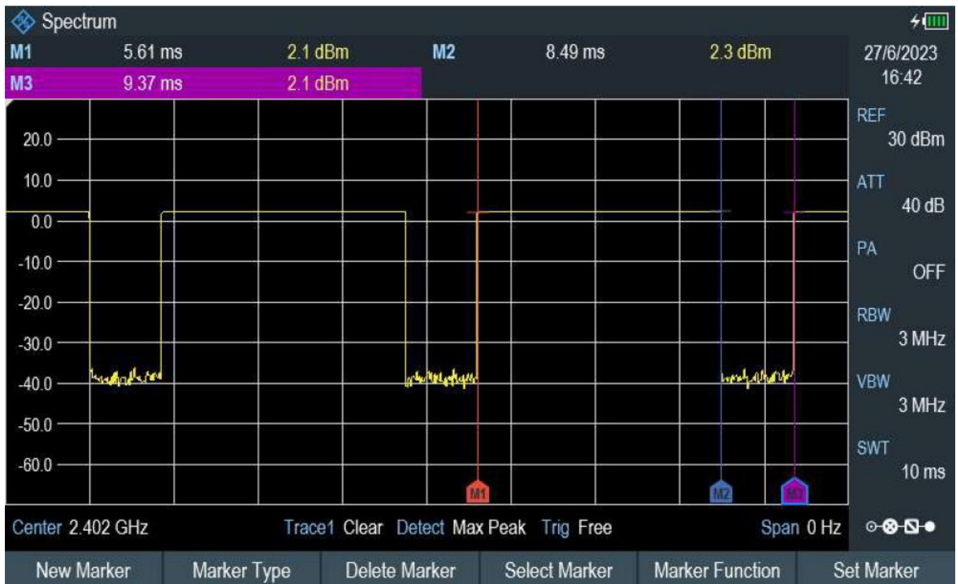
Time-domain plot for Bluetooth transmission signal
