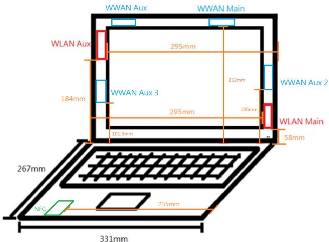
Photograph 5. Antenna position of EUT
