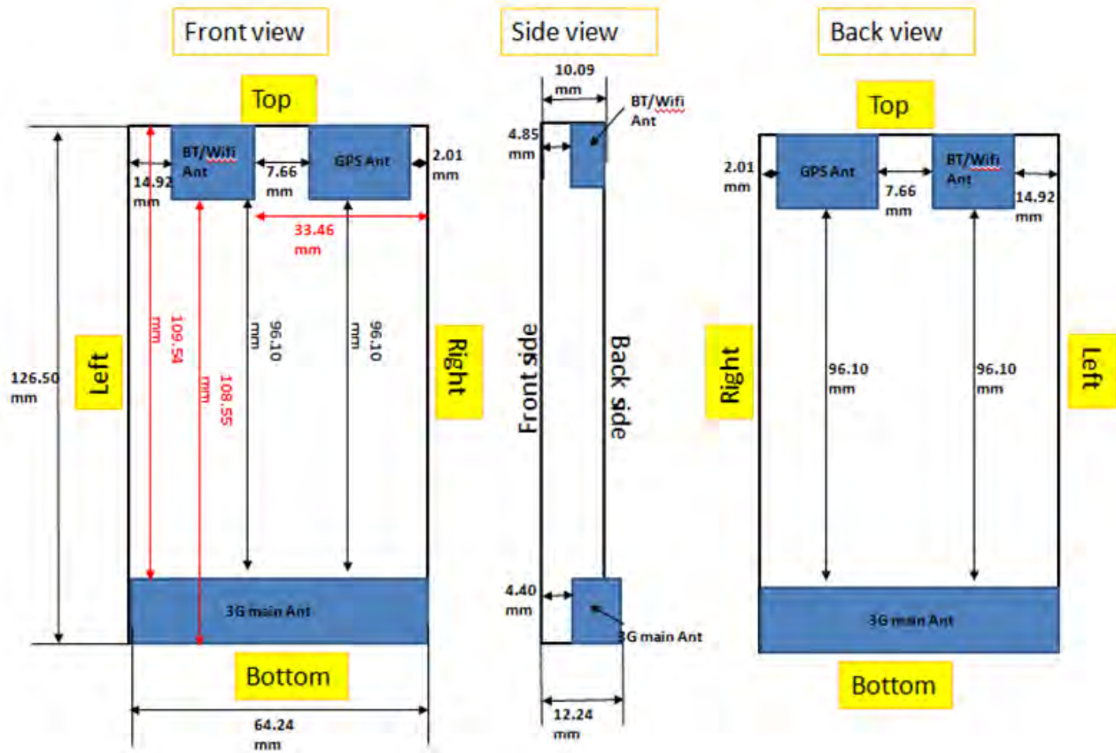
Fig.15 Antenna position & Antenna distance
