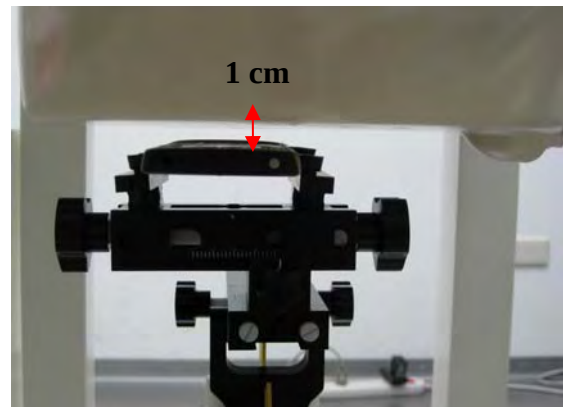
Fig.8 EUT rear to flat phantom
