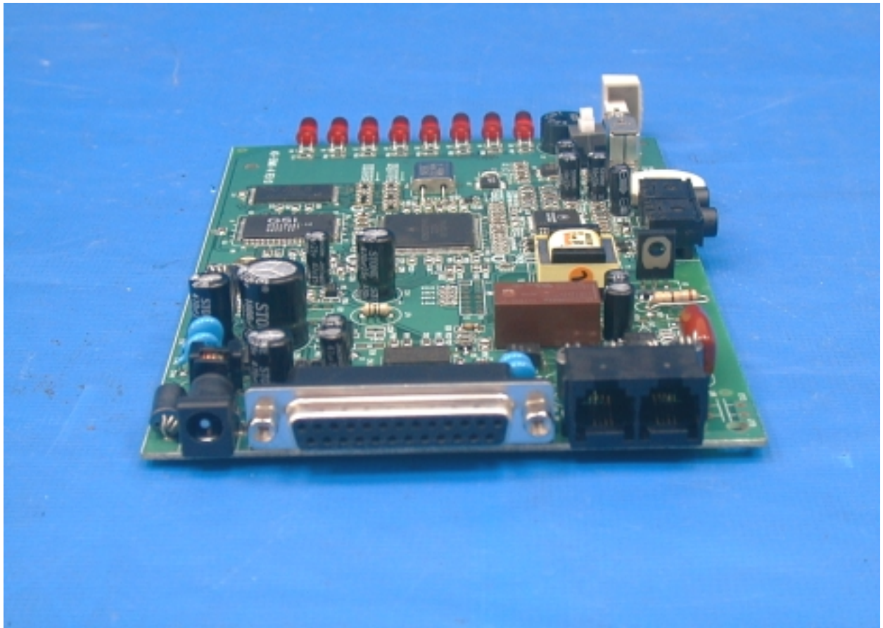
PHOTO. 7. EUT I/O PORT VIEW
