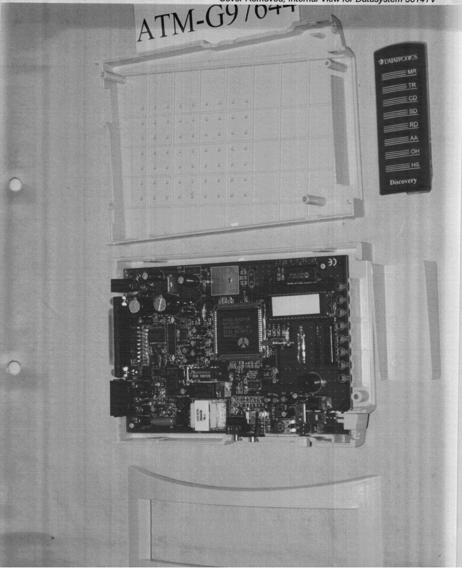
Figure 12 Cover Removed, Internal View for Datasystem 5614TV
