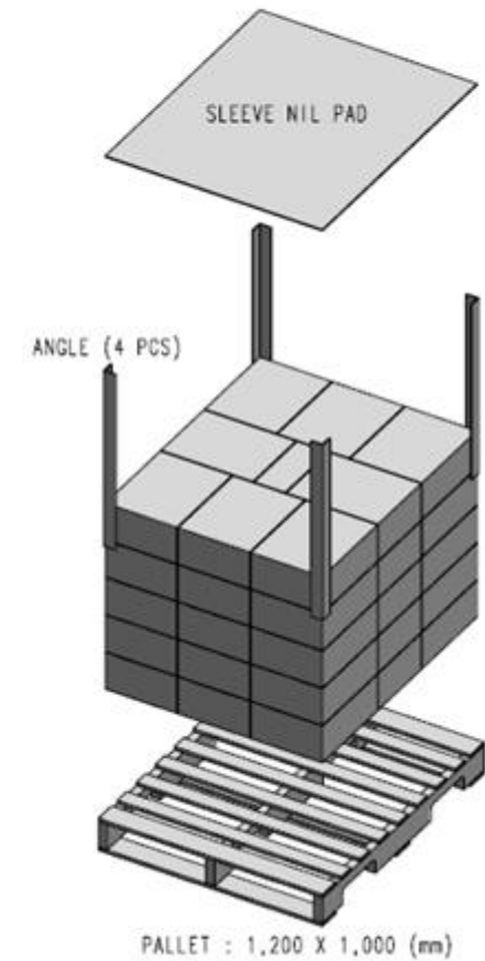
- PALLET PATTERN -
