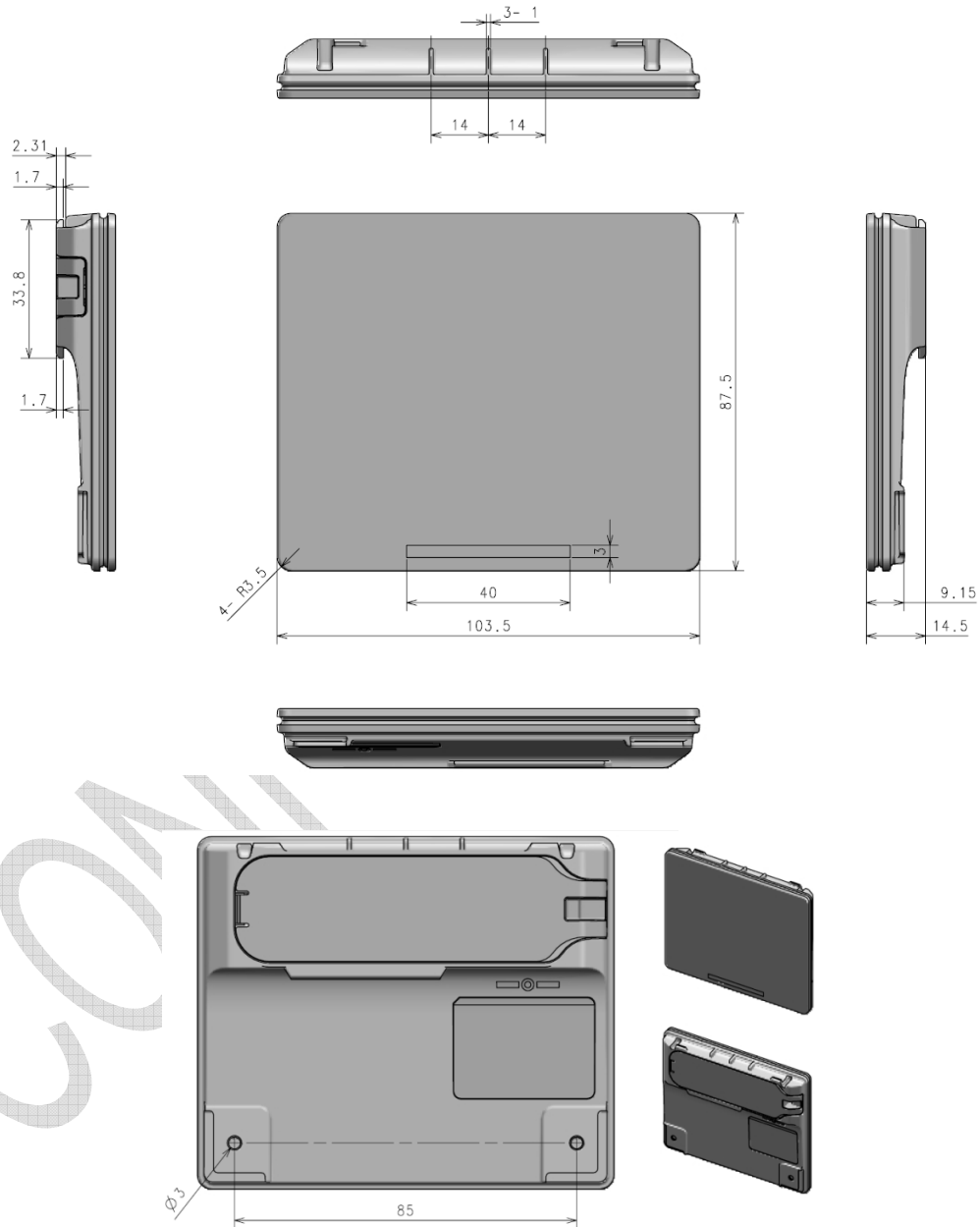
Figure 3 Mechanical Dimension
