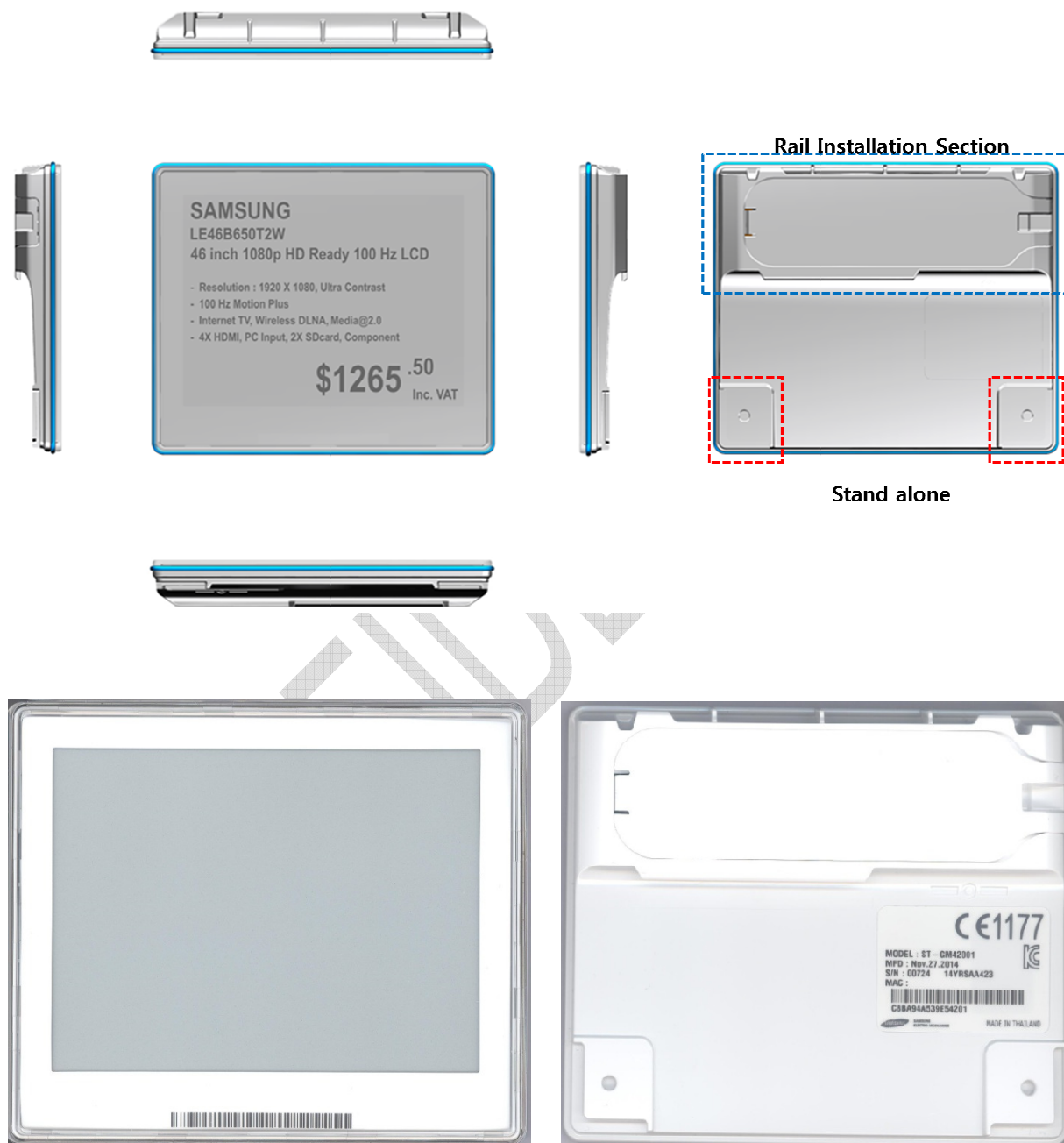
Figure 2 Appearance
