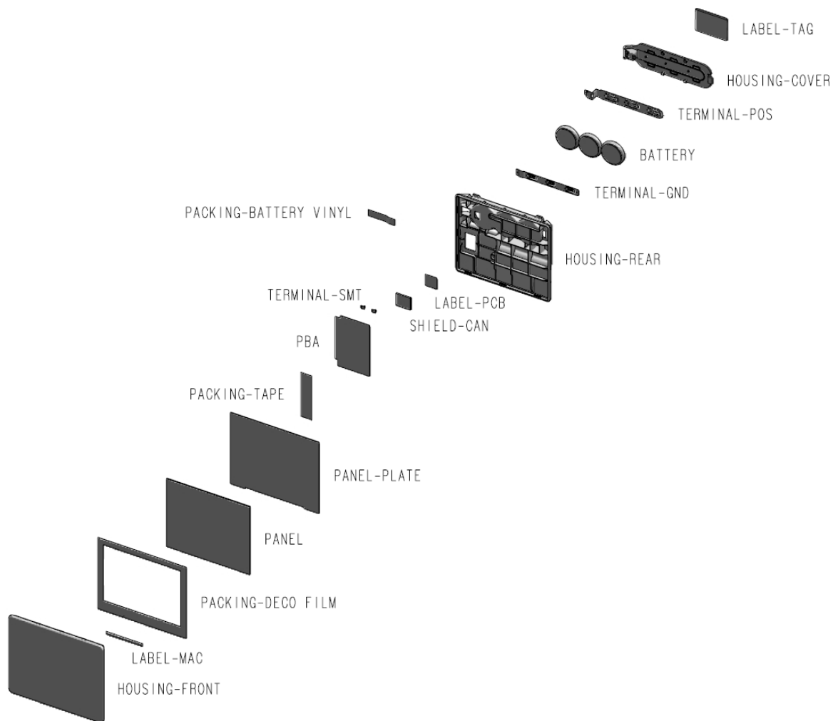
Figure 4 Exploded View
